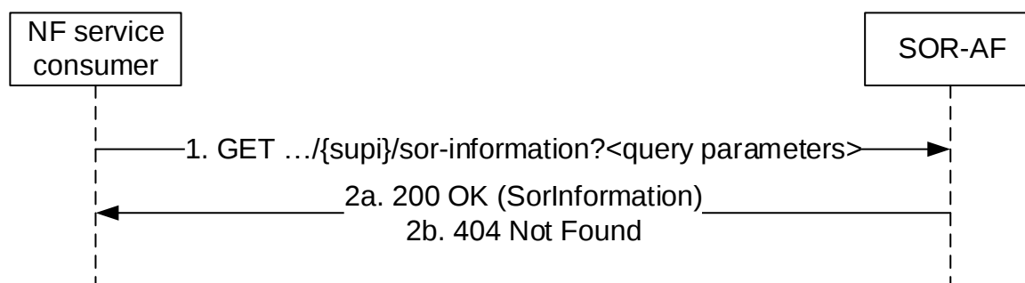
Figure 18: SoR Information Retrieval Procedure
