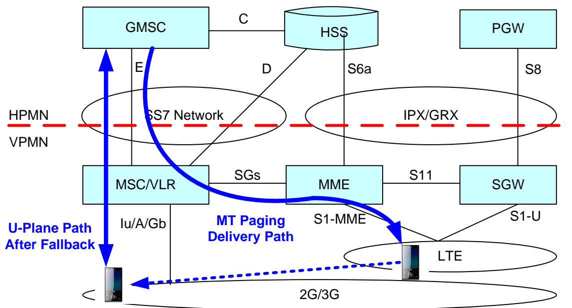
Figure 22: CSFB Roaming Architecture
