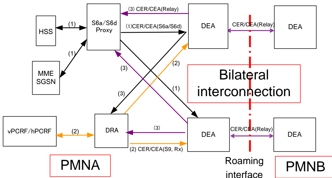
Figure 34: Diameter architecture example 1
