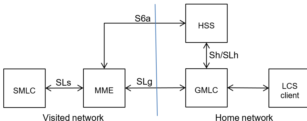
Figure 24 GMLC/MME/SLC architecture
