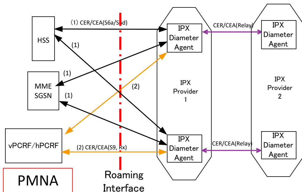
Figure 38: Diameter architecture example 6
