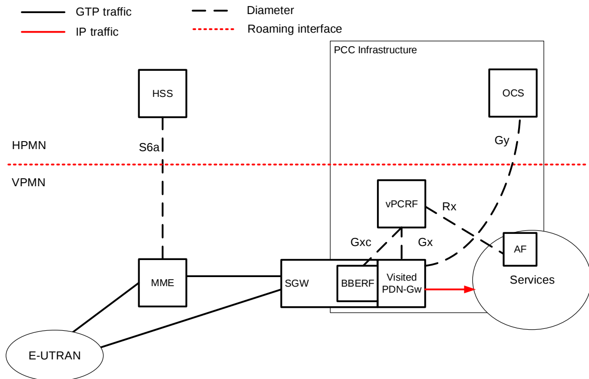
Figure 32: PCC Architecture with Local Break Out architecture
