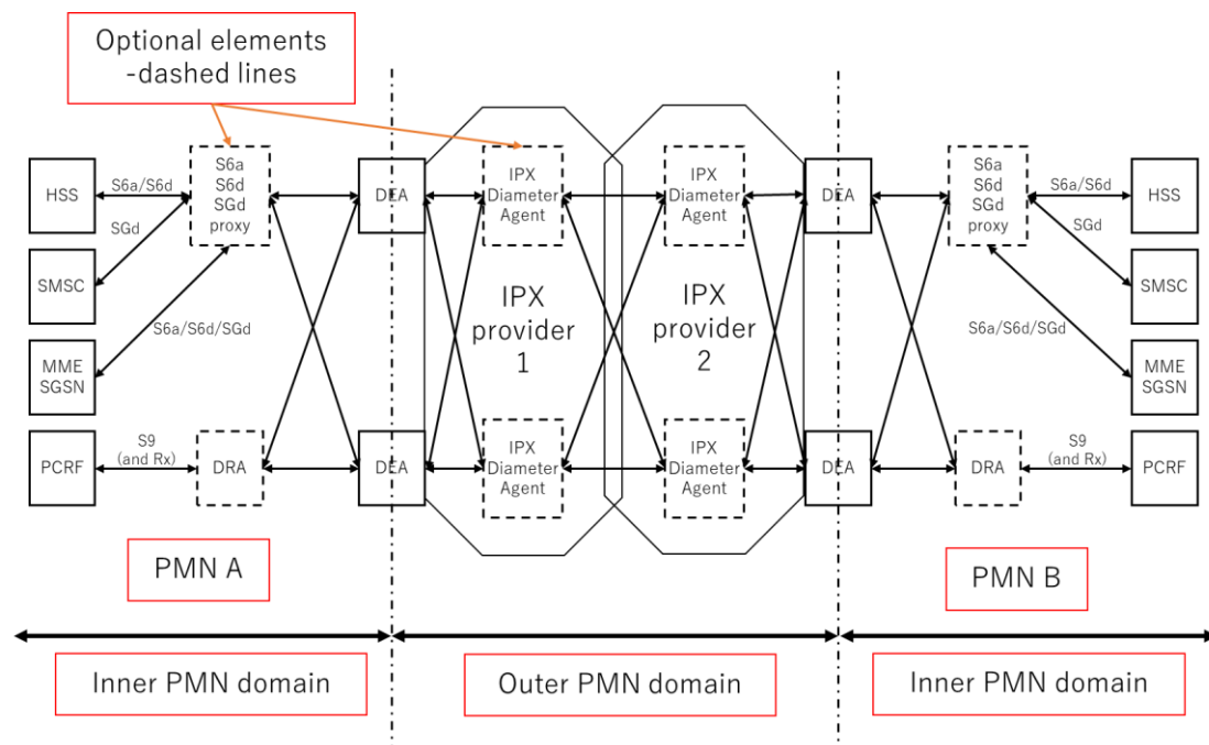
Figure 5: End to end Diameter Architecture
