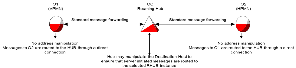
Figure 28: Direct connection
