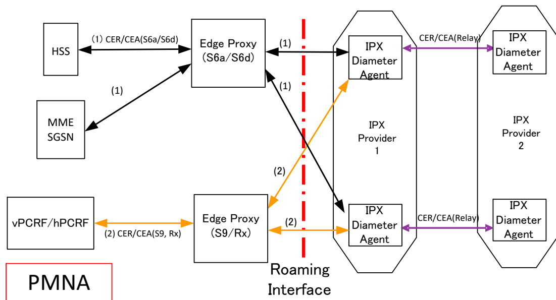
Figure 37: Diameter architecture example 5
