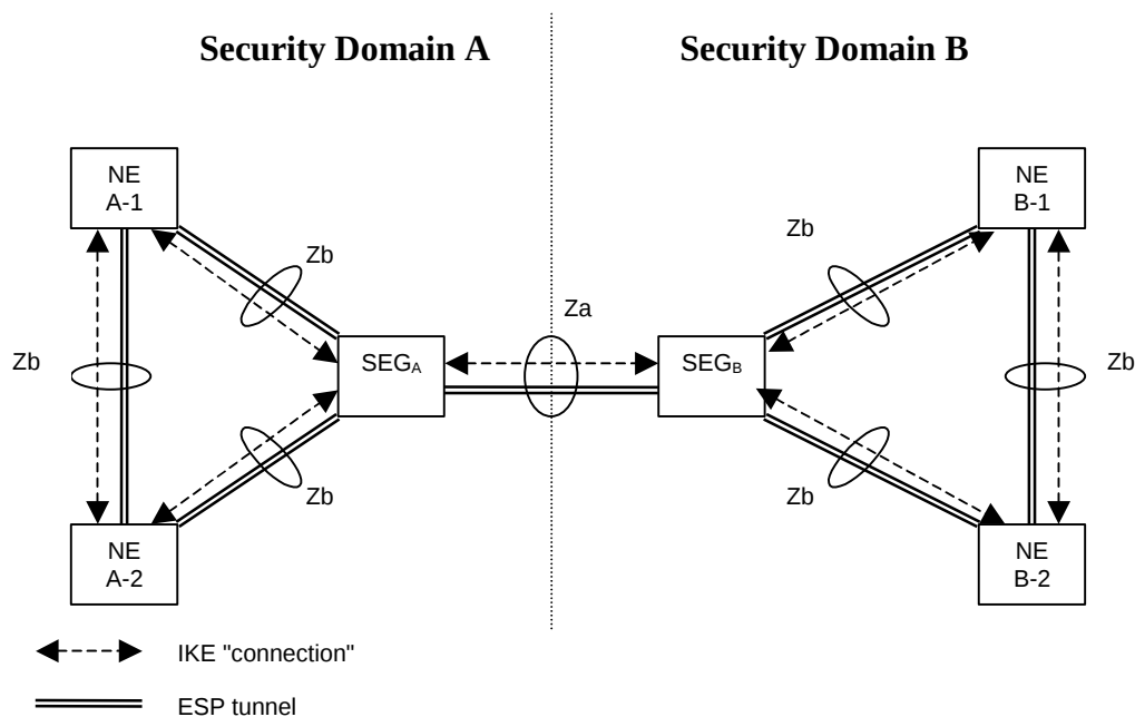
Figure 39: NDS/IP Architecture
