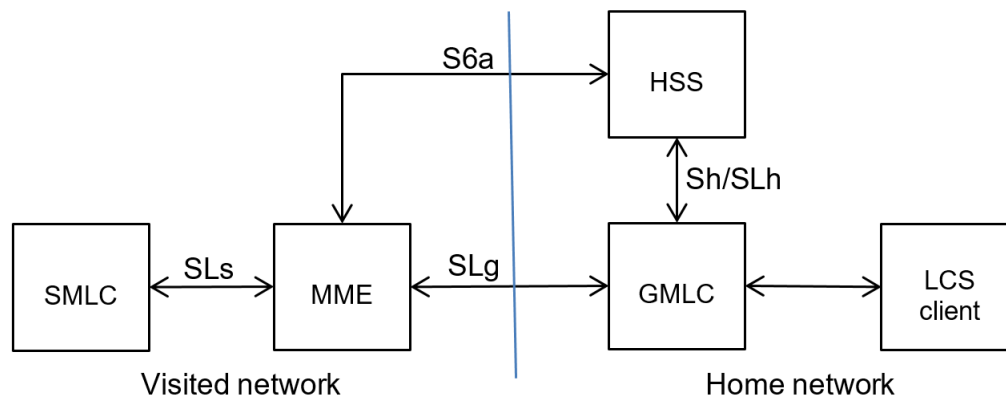
Figure 23 GMLC/MME/SMC architecture
