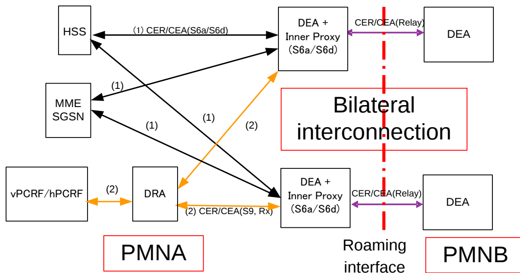
Figure 36: Diameter architecture example 4
