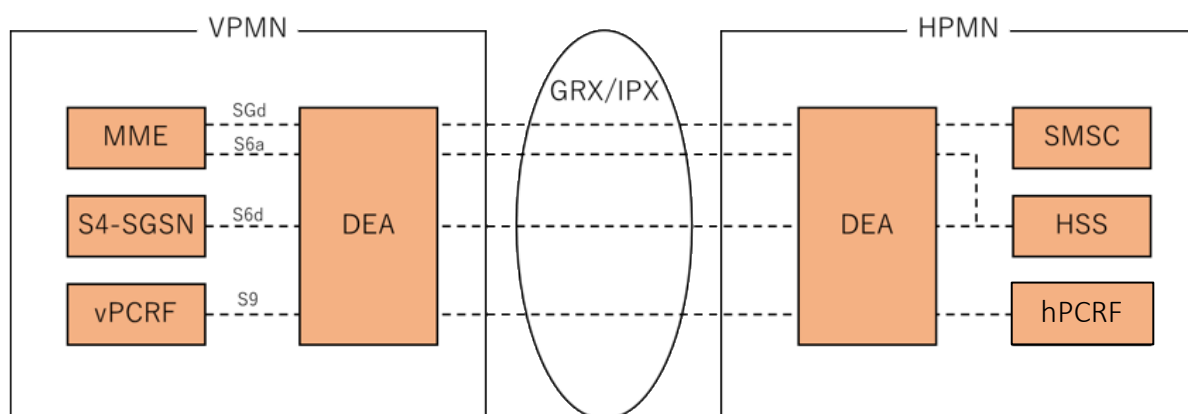
Figure 4: Diameter Roaming Implementation Architecture
