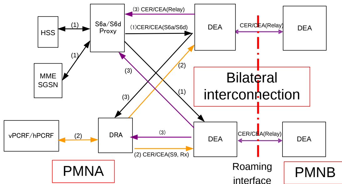
Figure 33: Diameter architecture example 1
