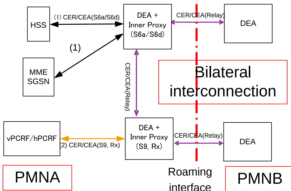
Figure 35: Diameter architecture example 3
