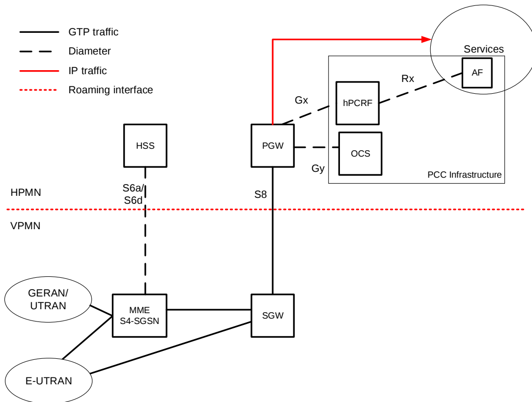
Figure 31: PCC Architecture with Home Routed architecture
