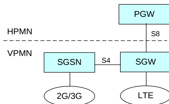
Figure 13: Scenario 3 - HPMN has only PGW as the gateway for roaming, 2G/3G Access via S8 interface
