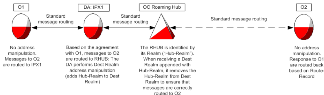
Figure 30: Destination realm modification
