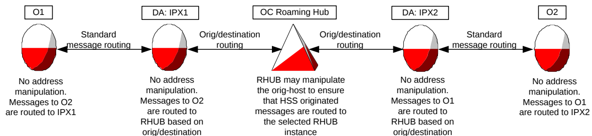
Figure 29: Origin/Destination realm based routing
