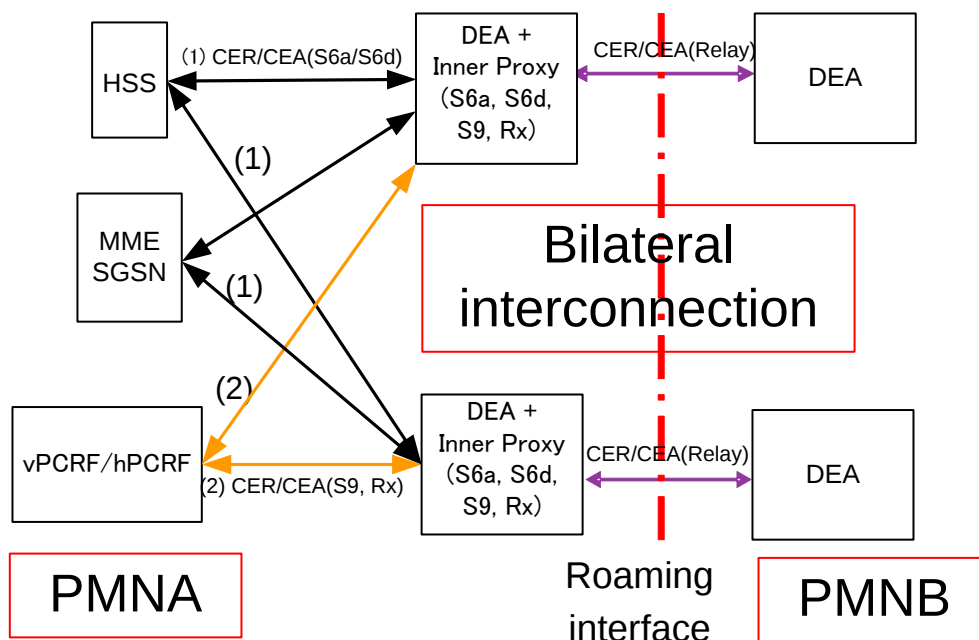
Figure 34: Diameter architecture example 2
