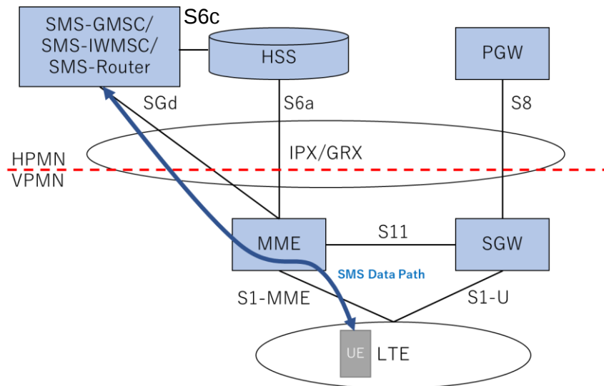
Figure 21: SMS in MME Roaming Architecture
