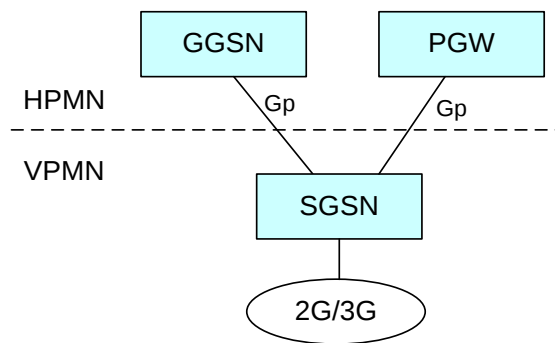
Figure 10: Scenario 3 - HPMN has both GGSN and PGW as the gateway for roaming
