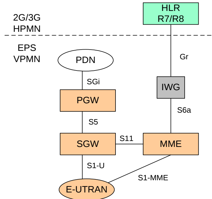
Figure 7: HPMN Legacy Roaming Architecture (local break-out)
