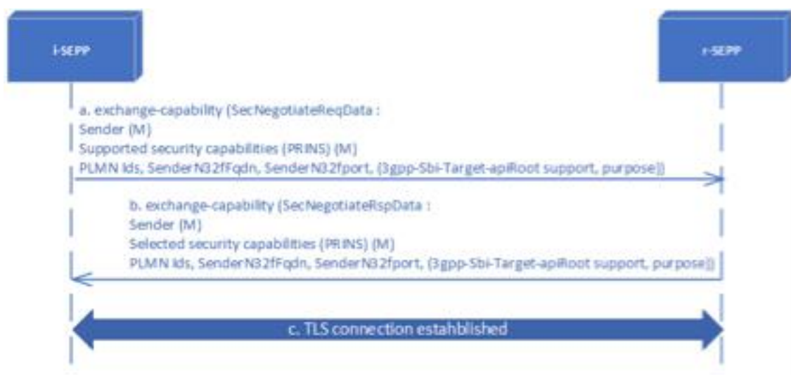
Figure 52 - N32-c Handshake
