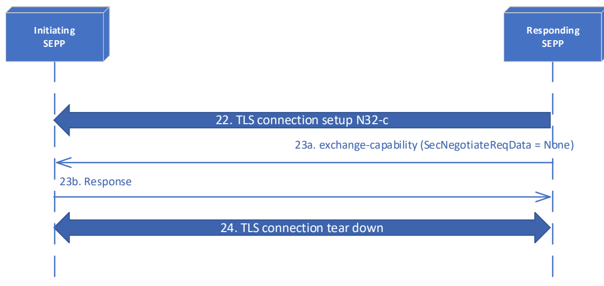
Figure 43 - N32 connection termination
