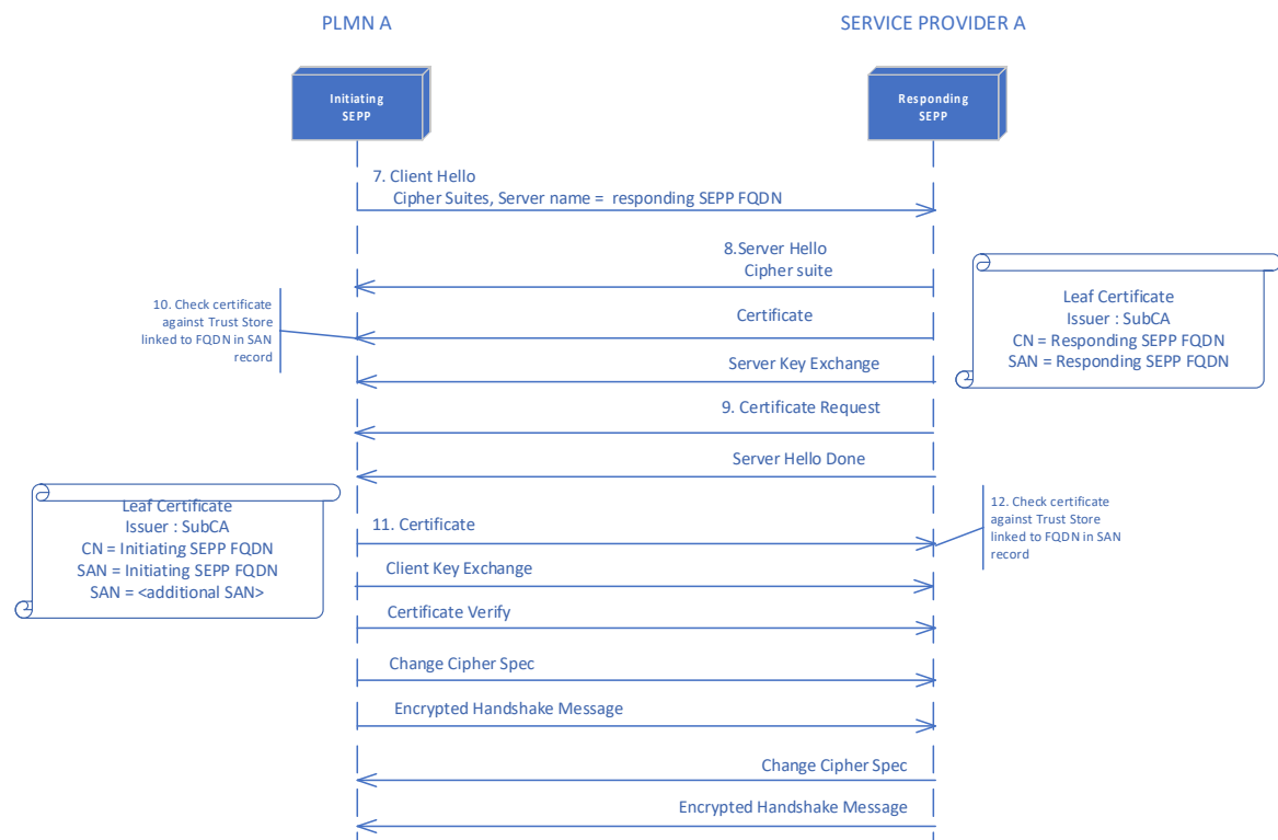
Figure 45 - TLS Handshake
