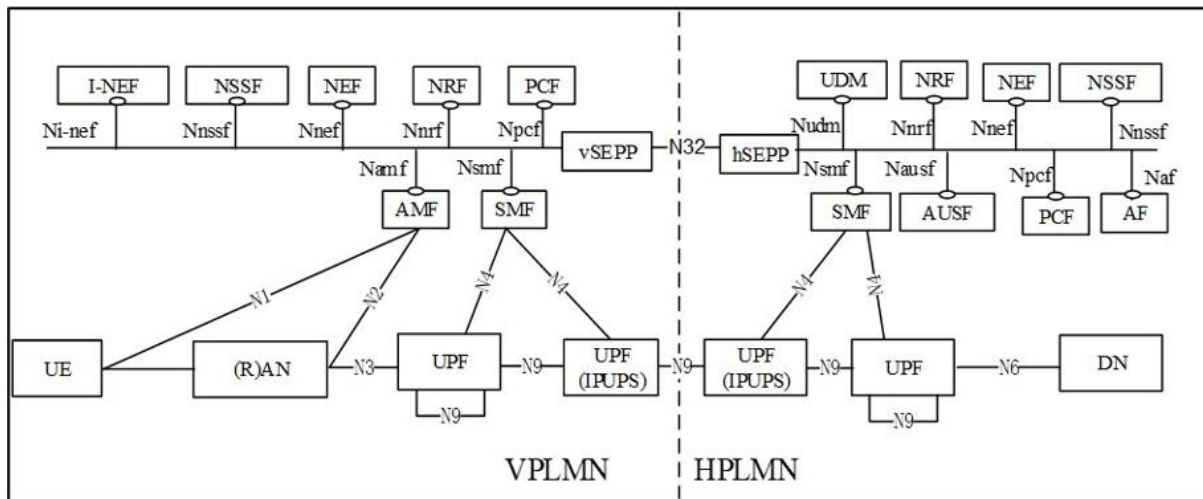
Figure 35 - Roaming Home Routing Scenario – In Serviced Based Interface Presentation
