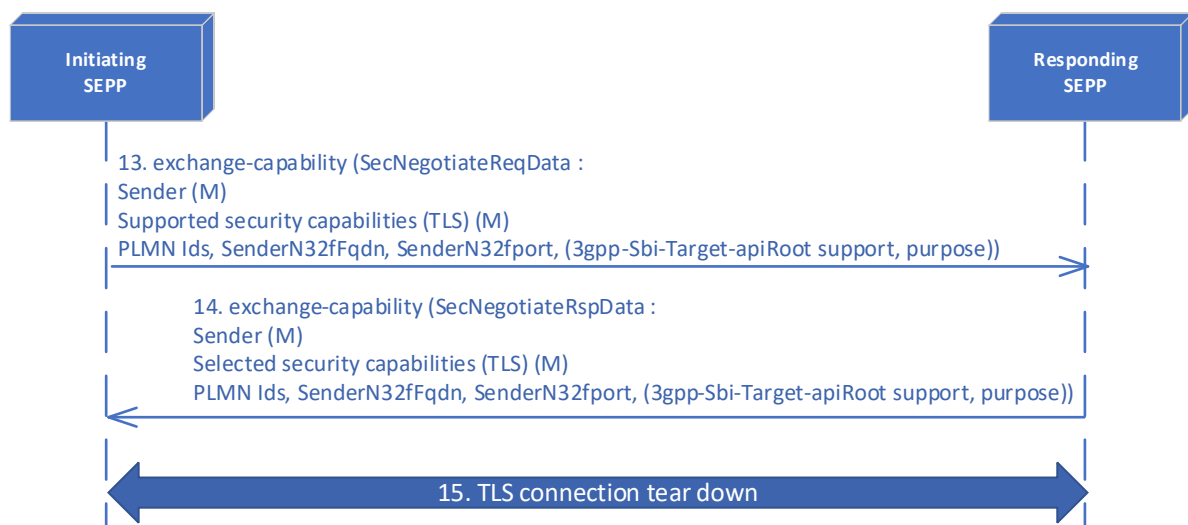
Figure 41 - N32-c Handshake
