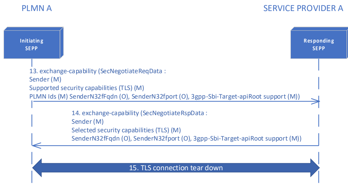
Figure 46 - N32s-c Handshake
