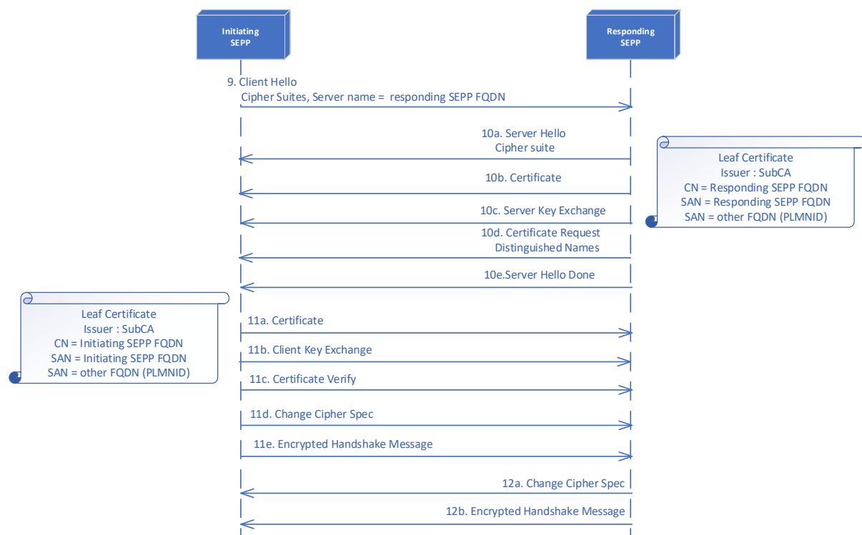
Figure 40 - TLS Handshake
