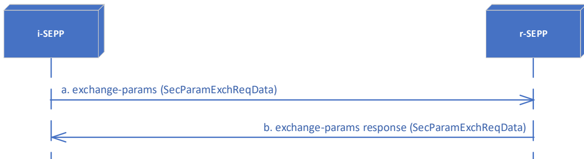
Figure 53 - N32-c Parameter Exchange
