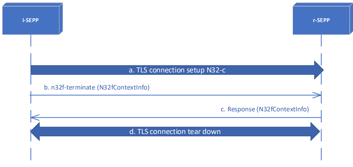
Figure 55 - N32-f Context Termination
