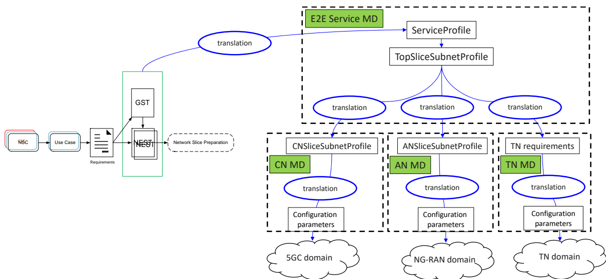
Figure 5 Relation between GST, 3GPP NRM ServiceProfile and ETSI ZSM architecture
