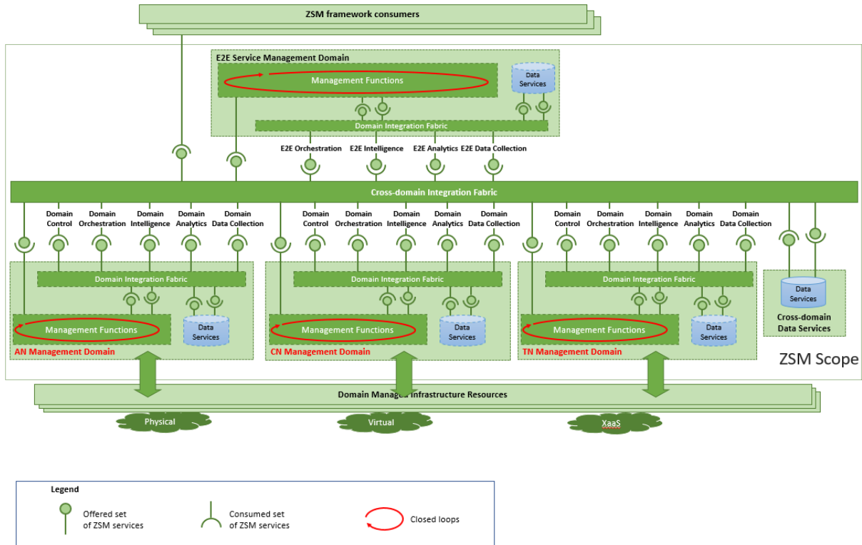
Figure 4 ZSM architecture deployment example for network slicing management [35]
