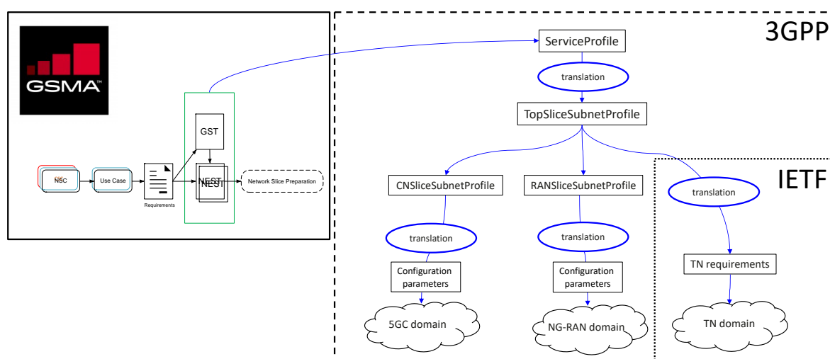
Figure 3: Relation between GST and network slice NRM ServiceProfile
