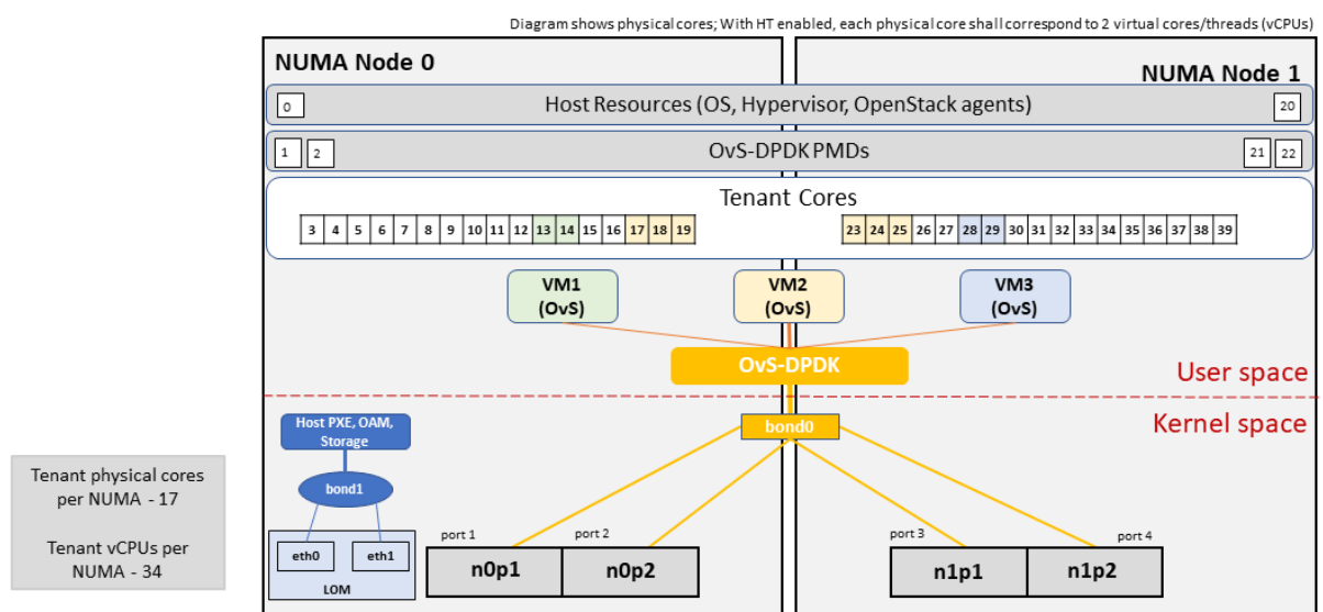
Figure 6 High Performance Profile Host Configuration with DPDK acceleration (example and simplified)
