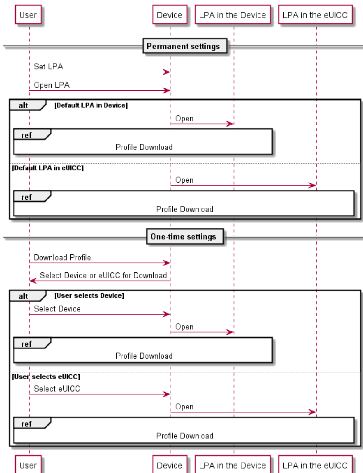
Figure 35: LPA Settings
