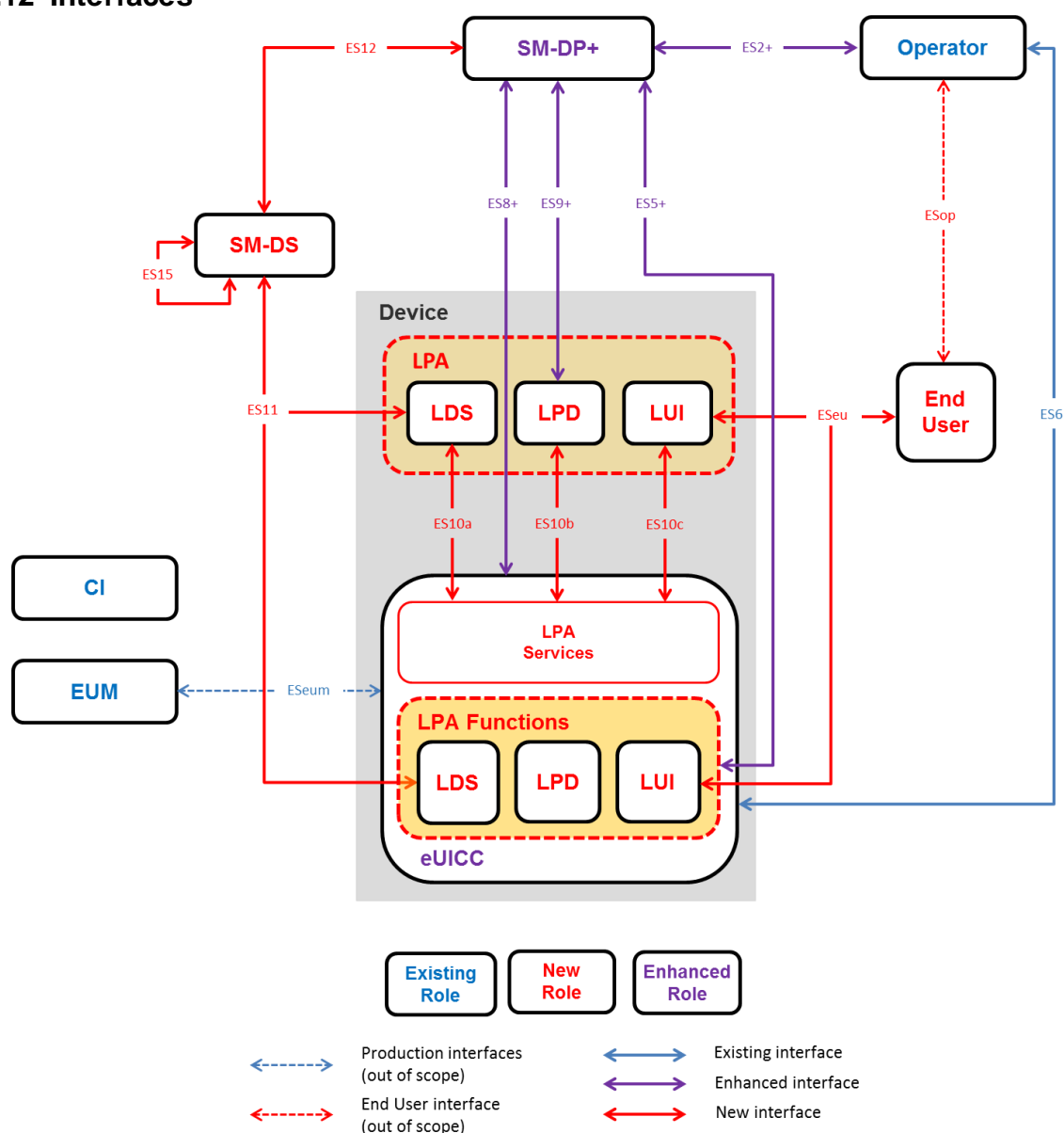
Figure 15: Interfaces on the eUICC Architecture with the LPA in the Device Configuration
