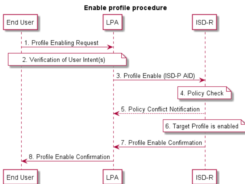
Figure 19: Enable Profile Procedure
