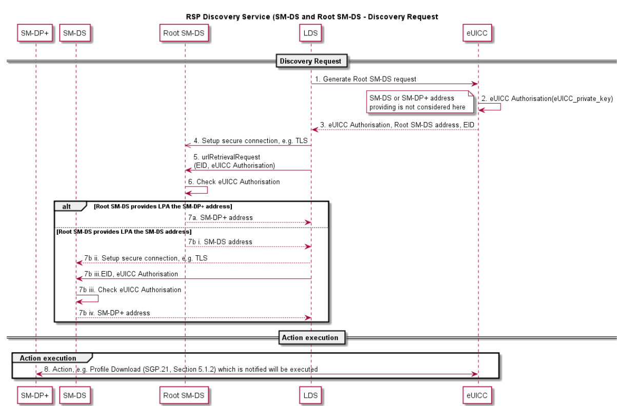
Figure 14: Discovery Request Procedure
