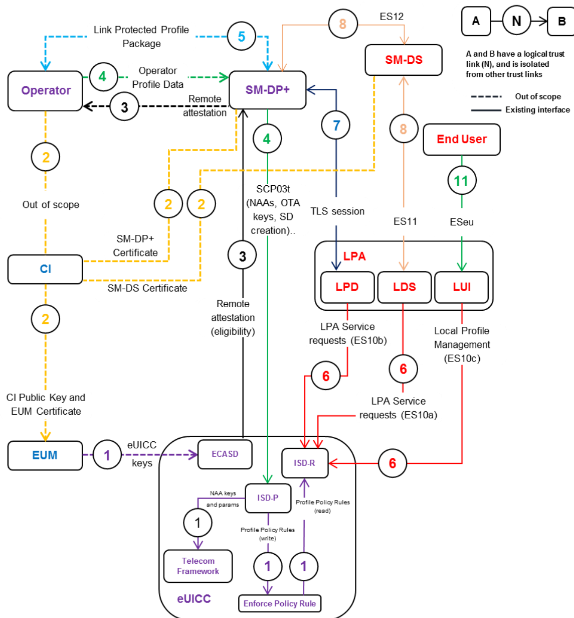
Figure 38: Trusted Link with LPA in the Device
