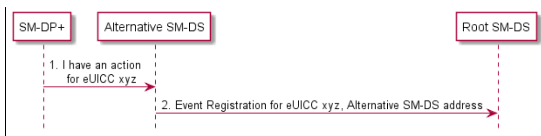
Figure 8: Alternative Device to Root SM-DS Event Registration
