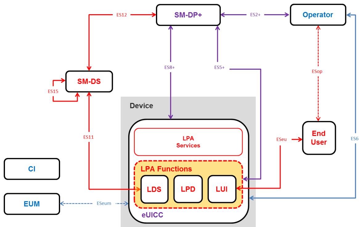
Figure 6: LPA in the Euicc
