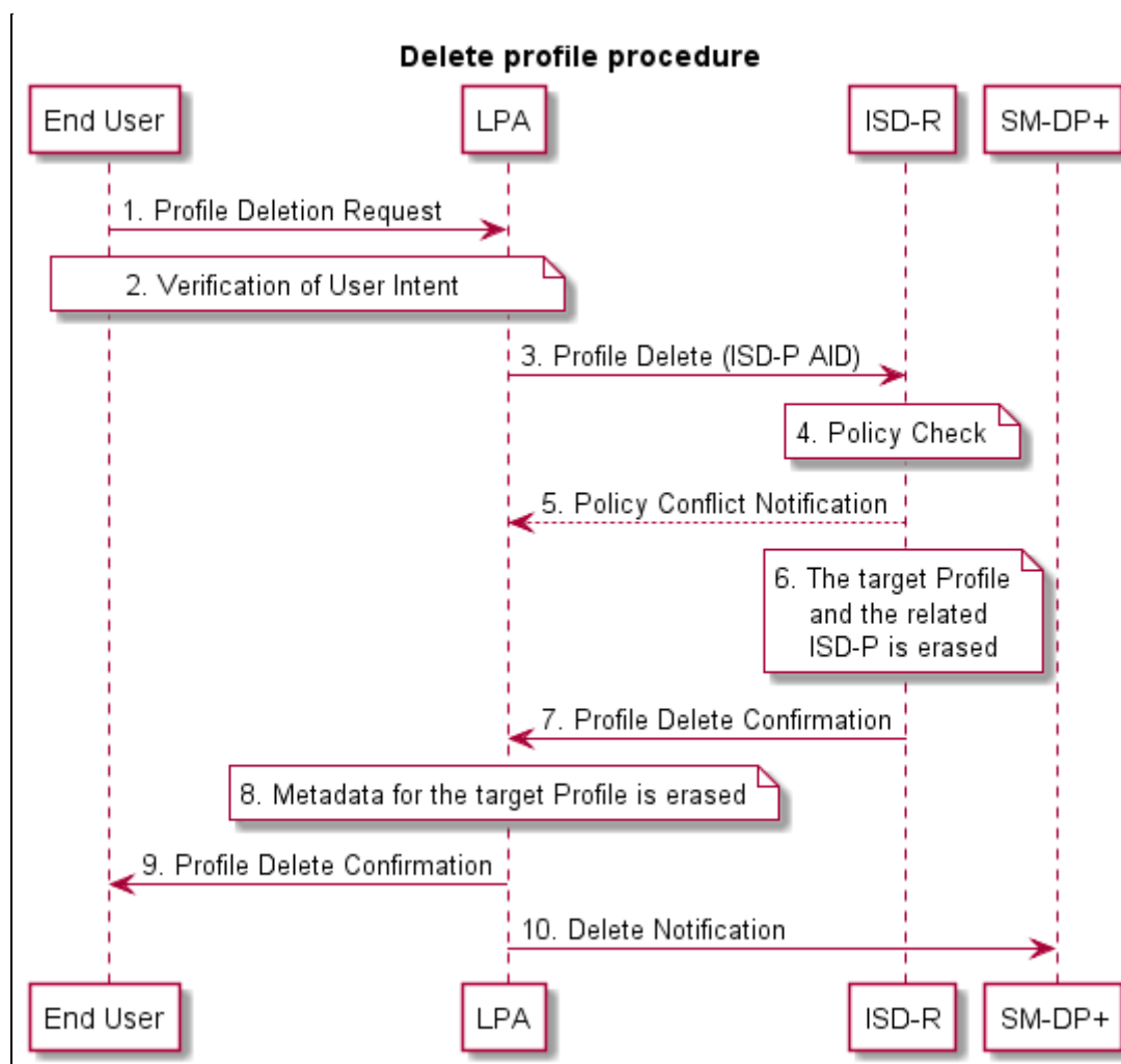
Figure 21: Delete Profile Procedure
