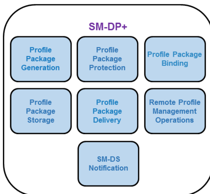
Figure 3: SM-DP+ Functions
