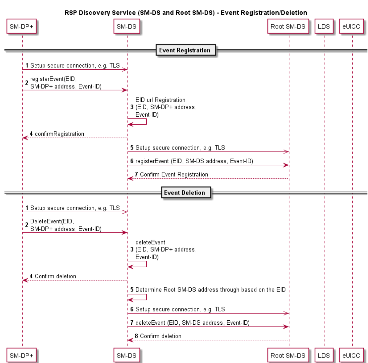
Figure 13: Event Registration/Deletion Procedure
