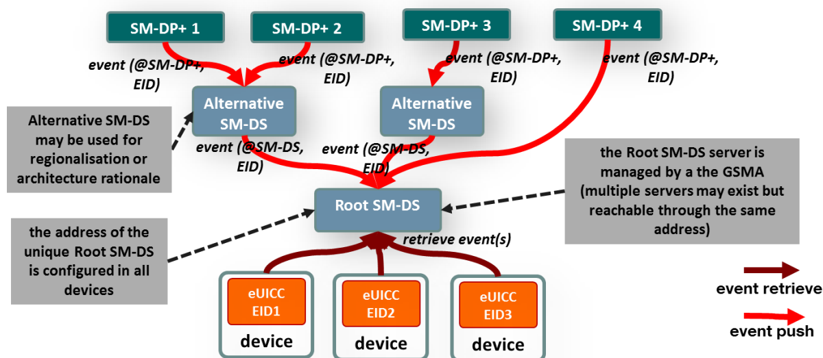
Figure 11: SM-DS Implementation
