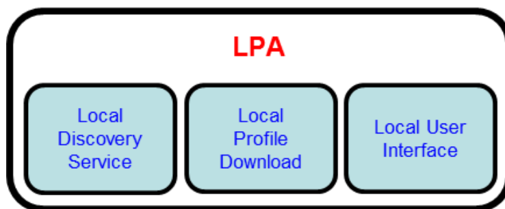
Figure 5: LPA Functions
