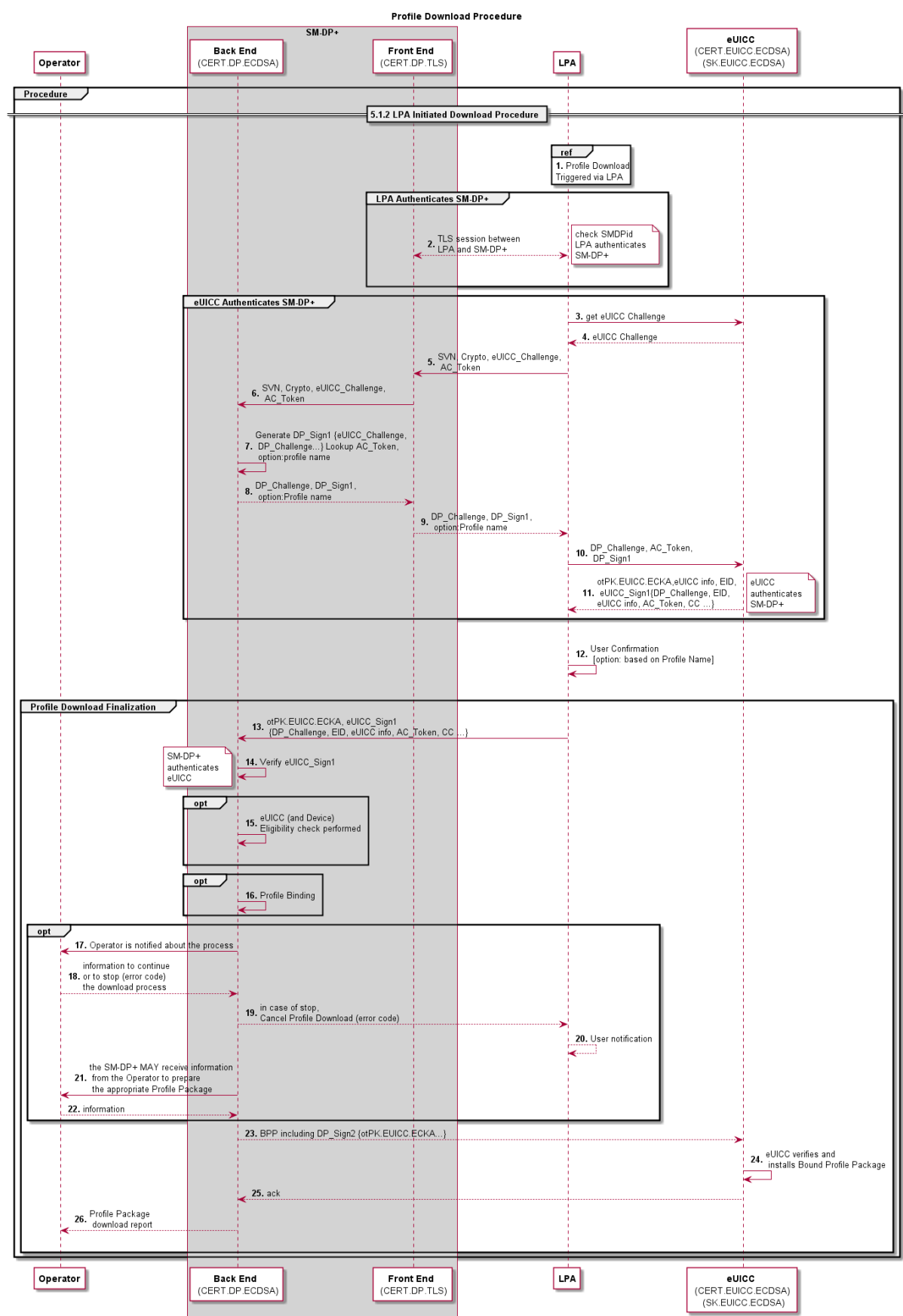
Figure 17: Profile Download Procedure
