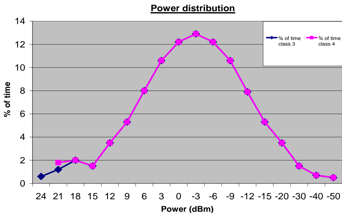
Figure 1: Terminal Tx Power distribution for WCDMA
