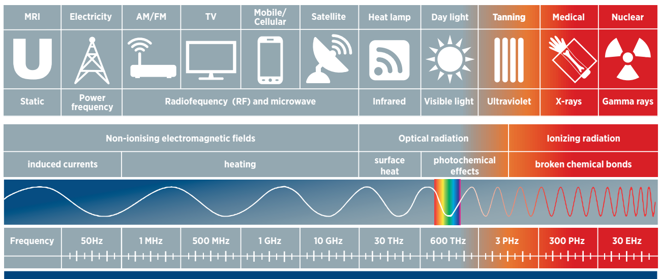
The Electromagnetic Spectrum
