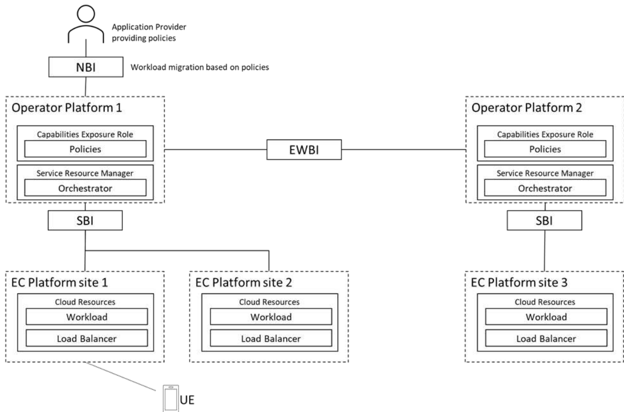
Figure 8: Serverless architecture
