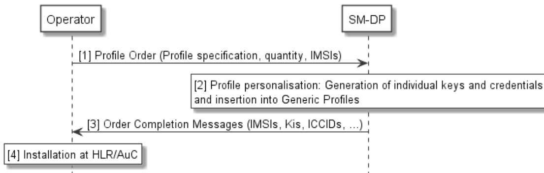
Figure 5: Profile Ordering
