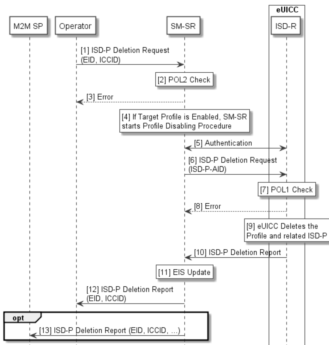
Figure 11: ISD-P Deletion
