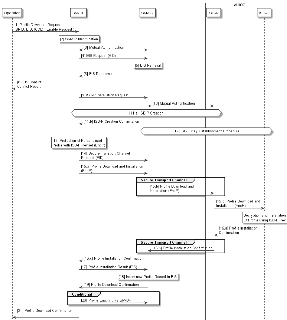
Figure 6: Profile Download
