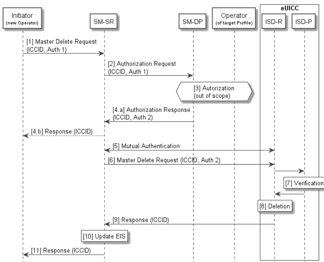
Figure 7: Master Delete
