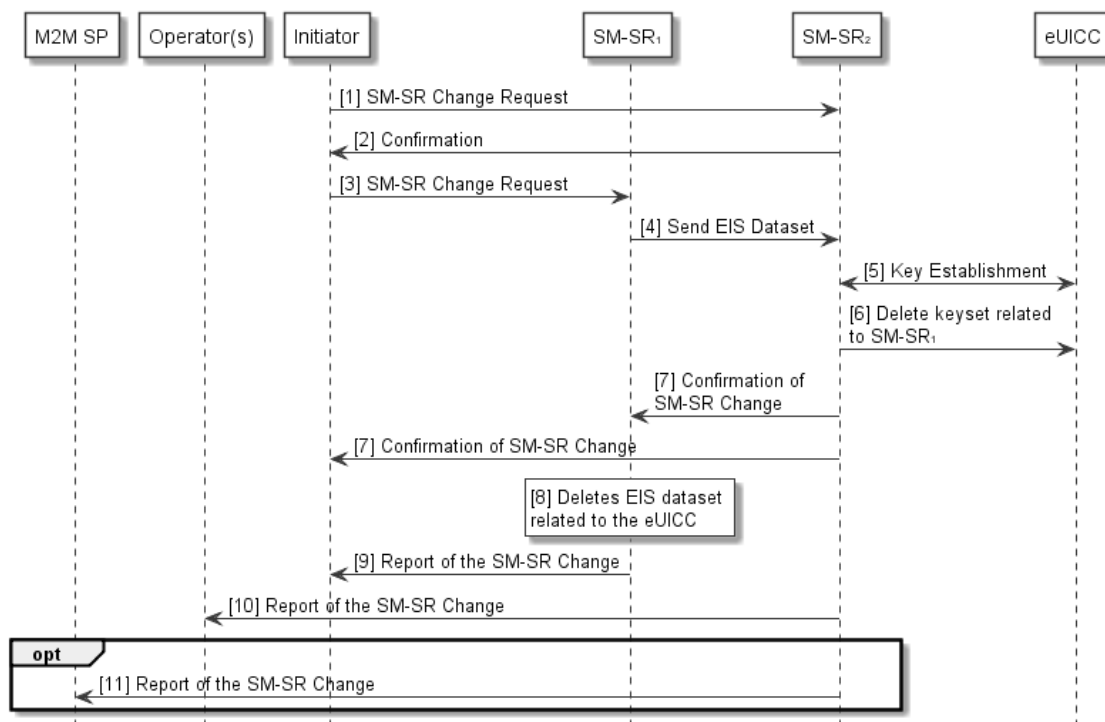
Figure 13: SM-SR Change
