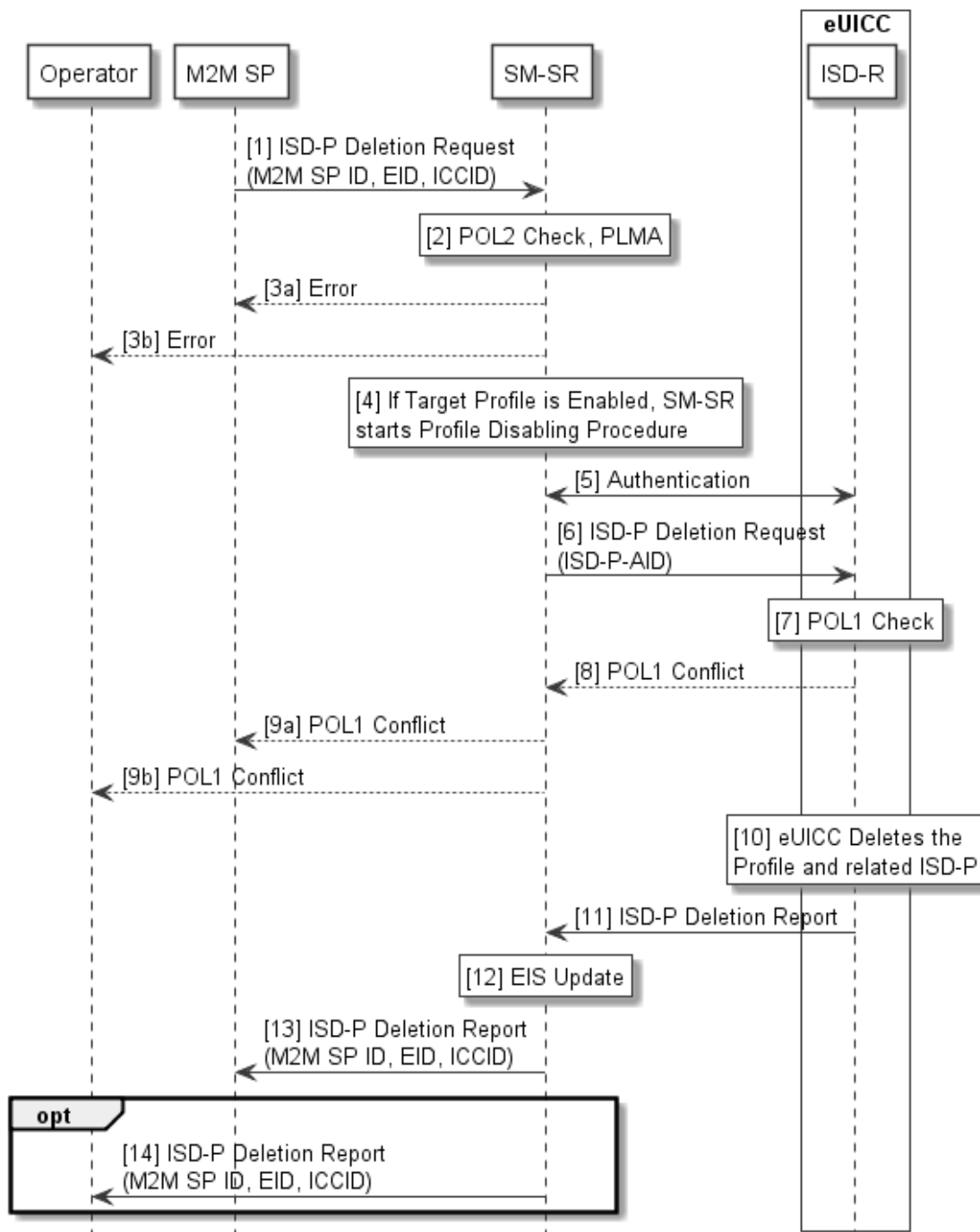
Figure 20: ISD-P Deletion via M2M SP
