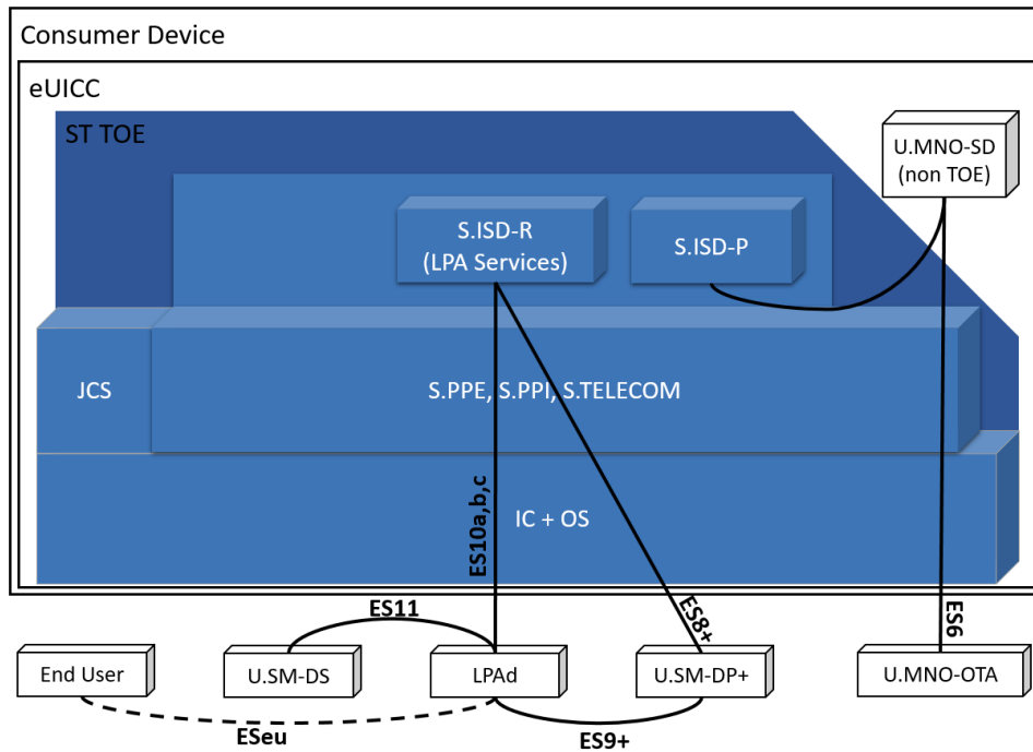
Figure 1 TOE Interfaces-LPAd
