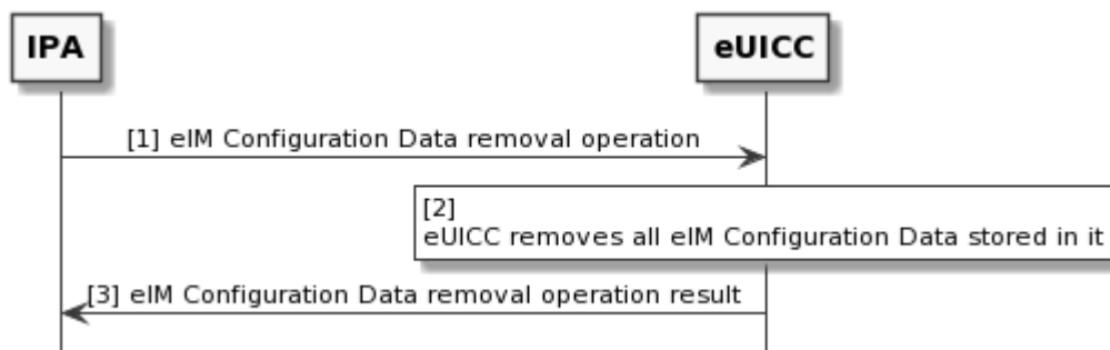
Figure 6.5.3.1: Complete Removal of eIM Configuration Data from the eUICC
