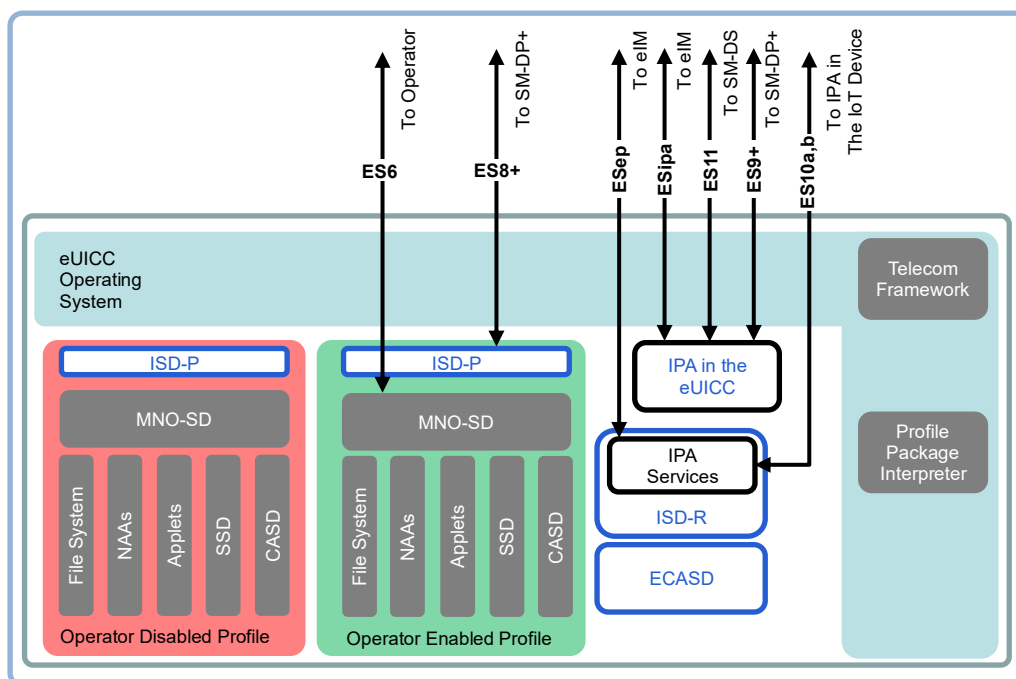
Figure 4.3.1.1: eUICC Architecture (IPA in eUICC)
