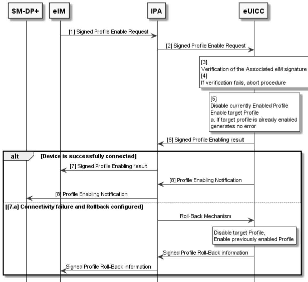
Figure 6.2.1.1: Profile Enabling via eIM
