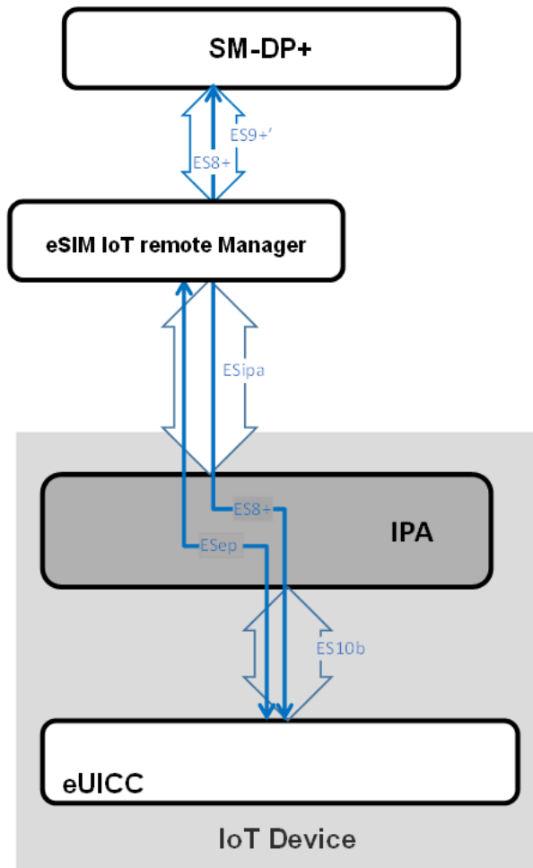
Figure C.1.1.1: Indirect Profile download assisted by eIM using AC
