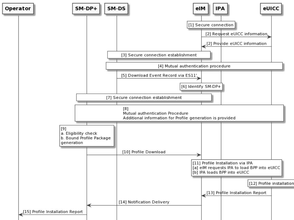
Figure 6.1.5.1: eIM Assisted Profile Download Triggered by eIM with SM-DS
