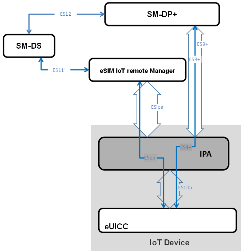
Figure C.2.2.1 Direct Profile Download assisted by eIM using SM-DS
