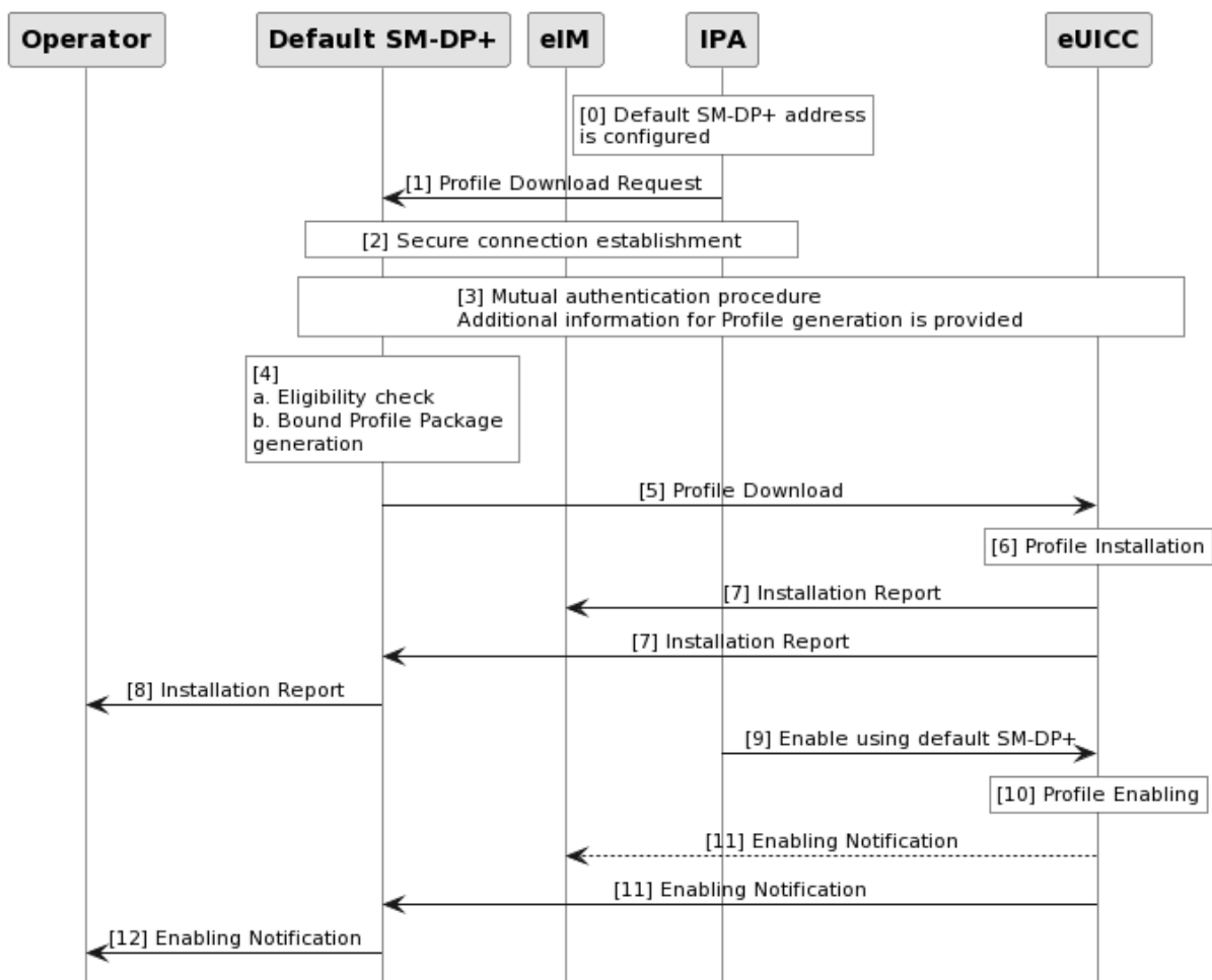
Figure 6.1.4.1: Profile Download with Default SM-DP+
