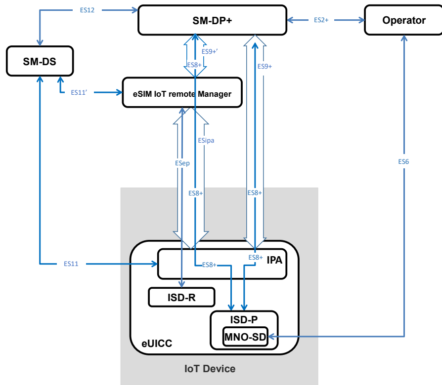
Figure 4.1.2.1: eSIM IoT Functional Architecture (IPA in the eUICC)
