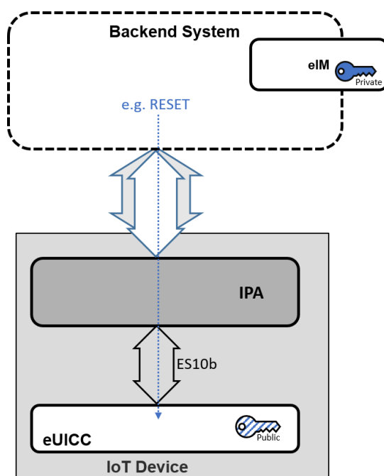
Figure B.5.1: Removal of eIM Configuration
