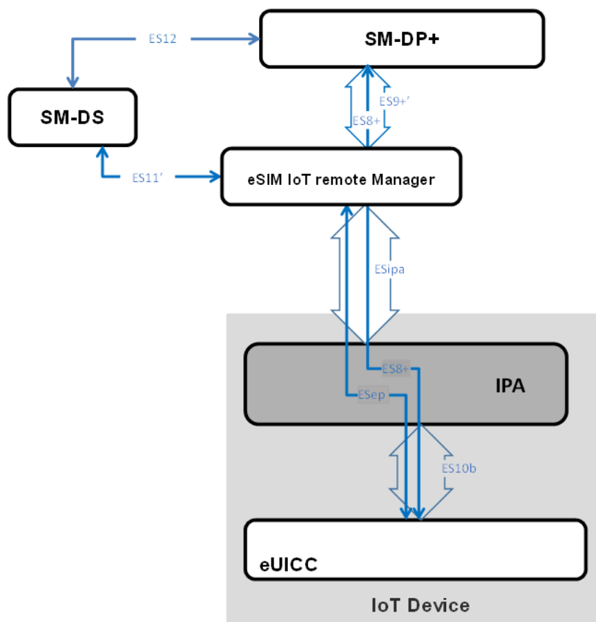
Figure C.1.2.1: Indirect Profile download assisted by eIM using SM-DS
