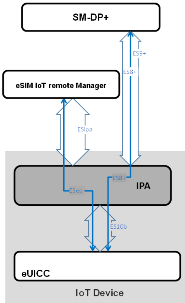
Figure C.2.1.1 Direct Profile Download assisted by eIM using AC
