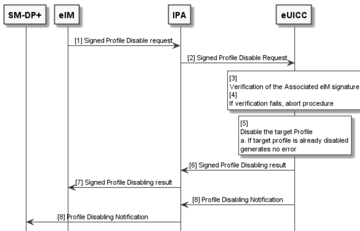
Figure 6.3.1.1: Profile Disabling via eIM
