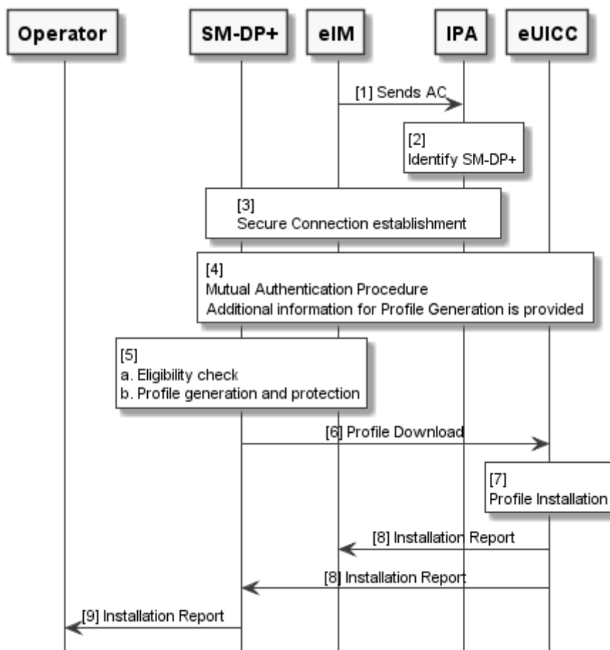
Figure 6.1.1.1: Profile Download Triggered by eIM with Activation Code
