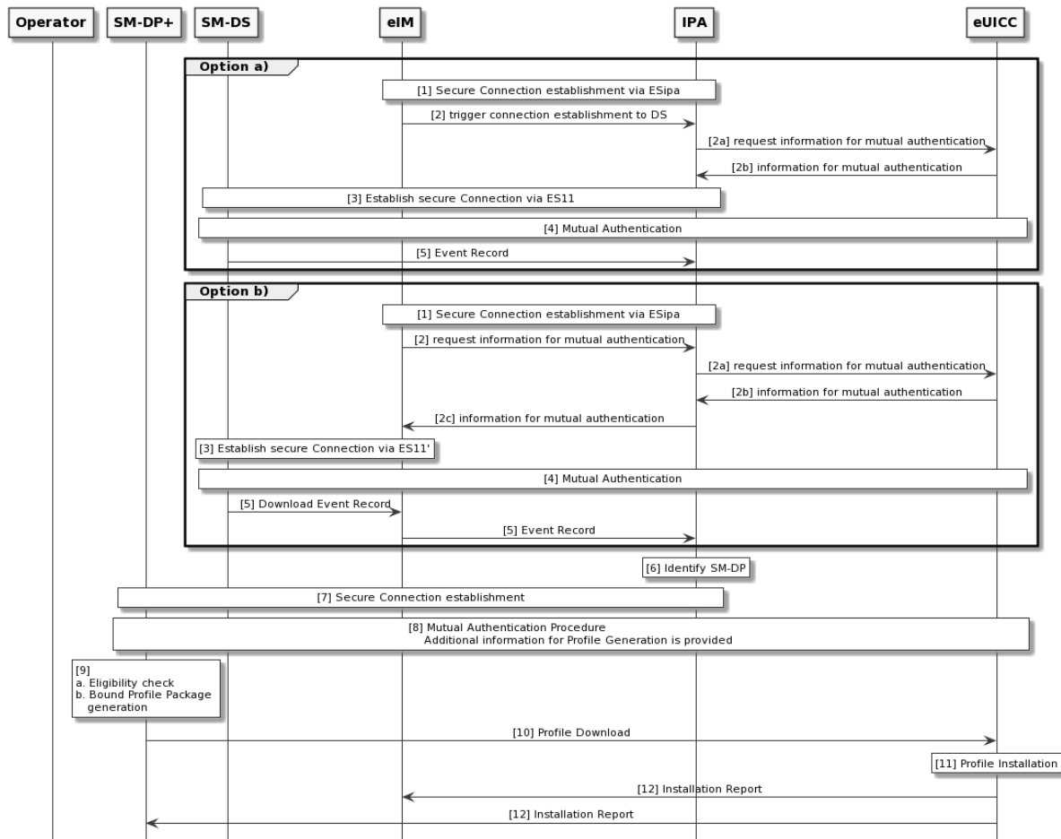
Figure 6.1.2.1: eIM Initiated Direct Profile Download with SM-DS
