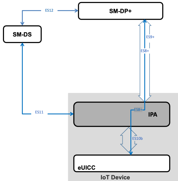
Figure C.2.3.1 Direct Profile download unassisted by eIM using SM-DS
