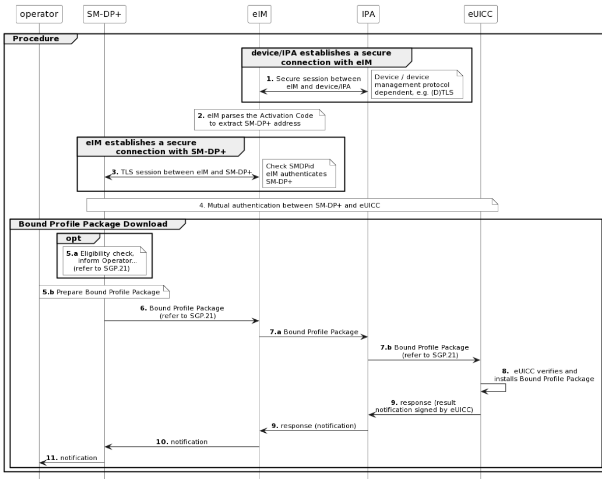
Figure 6.1.3.1: eIM Assisted Profile Download Triggered by eIM with Activation Code
