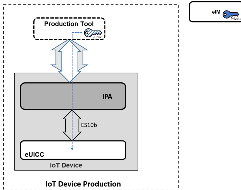
Figure B.2.1: eIM Configuration performed in IoT Device production
