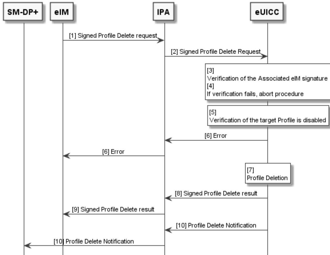
Figure 6.4.1.1: Profile Delete via eIM
