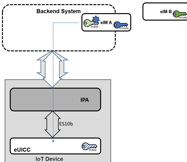
Figure B.4.1: eIM Configuration performed by an eIM
