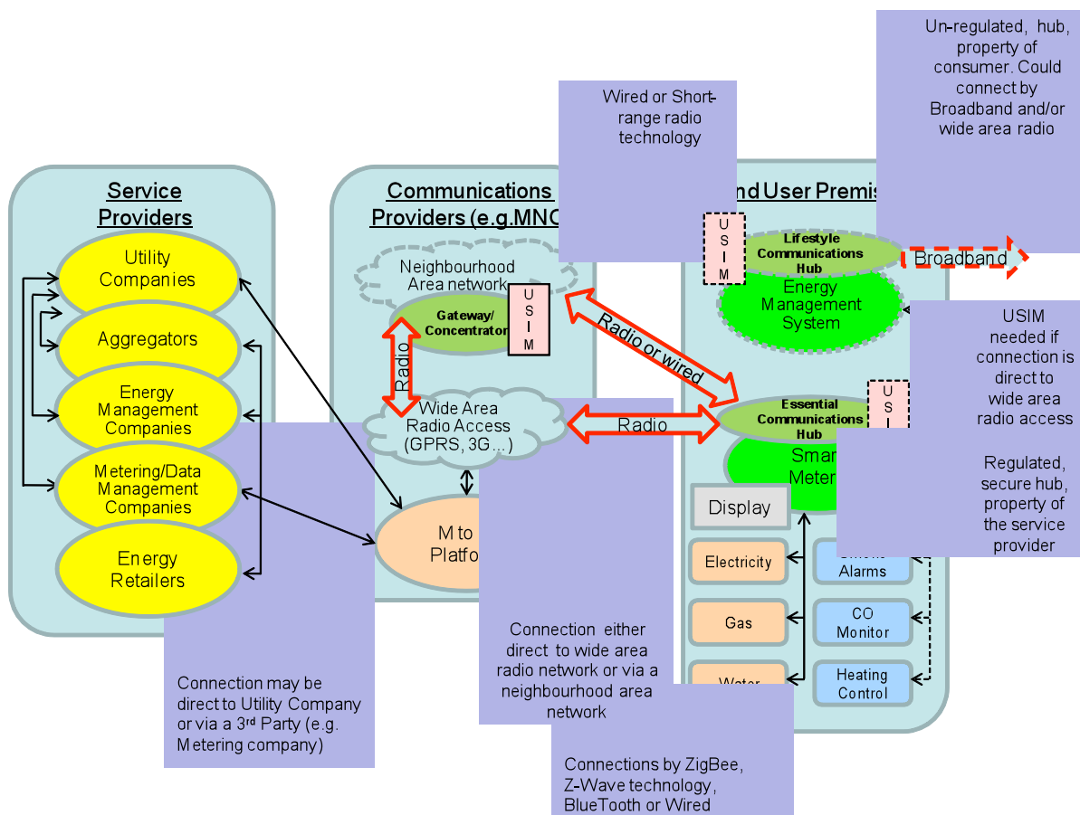
Figure 17 Architectural Relationships for Smart Metering Use Cases
