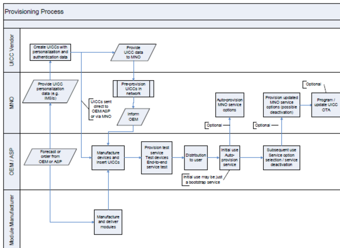
Figure 3 Provisioning Process Flow Example
