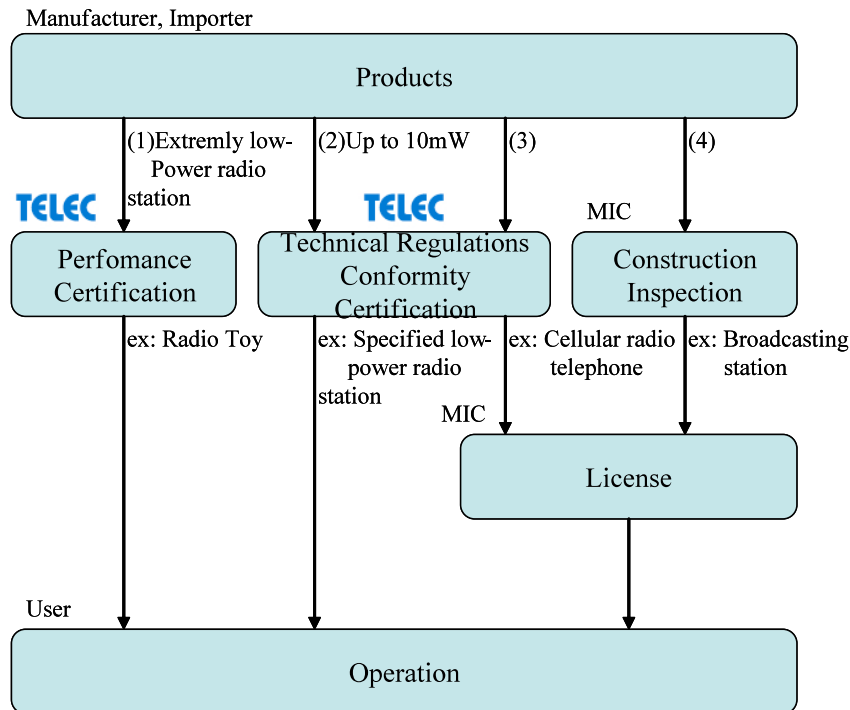
Figure 23 Certification process flow for radio products seeking approval in Japan.
