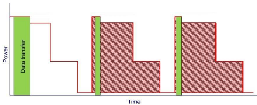
Figure 5: Power Consumption – Example 2
