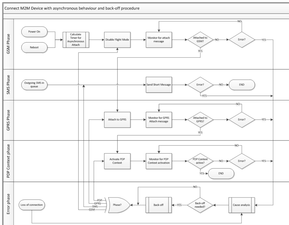
Figure 3: Logic Flow for Back Off Procedure
