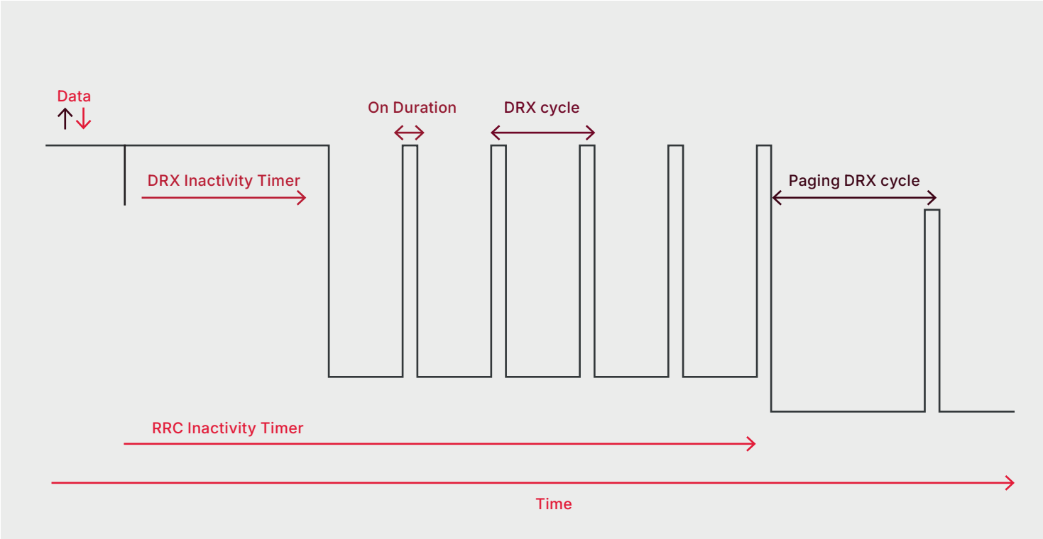
Figure 3, Connected-Mode (Extended) DRX Support
