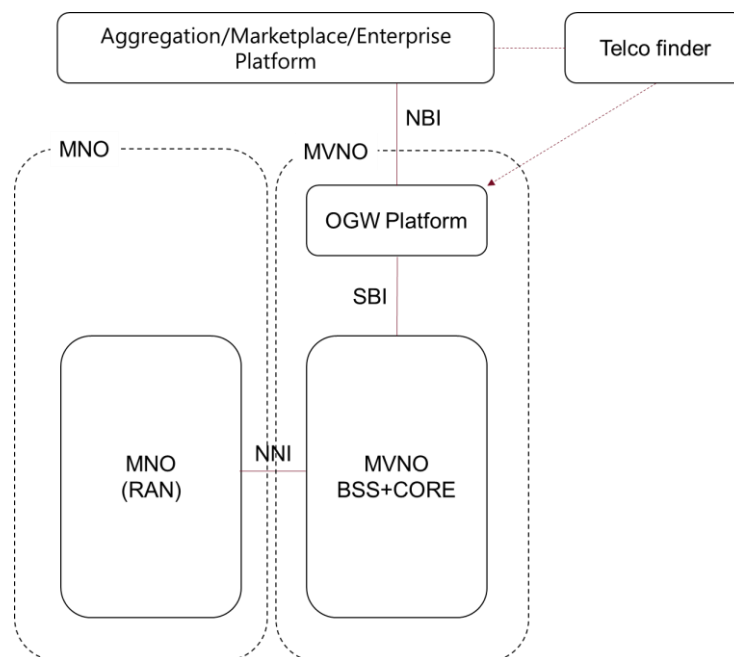
Figure 20 OGW Platform in Full MVNO
