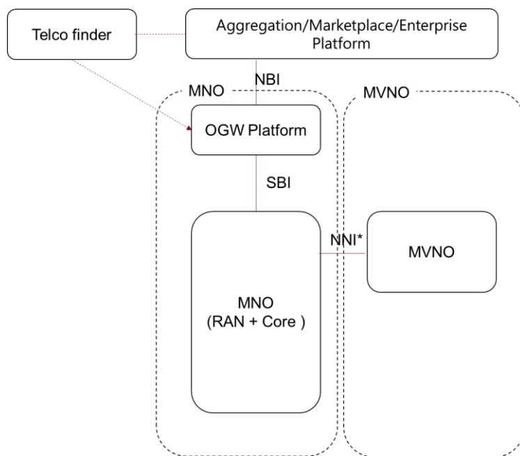
Figure 18 Reseller deployment
