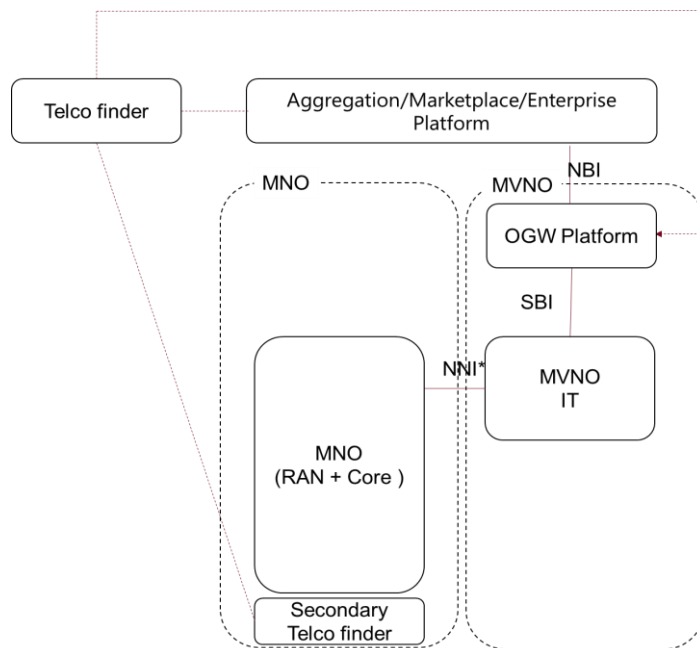
Figure 19OGW Platform in Thin MVNO
