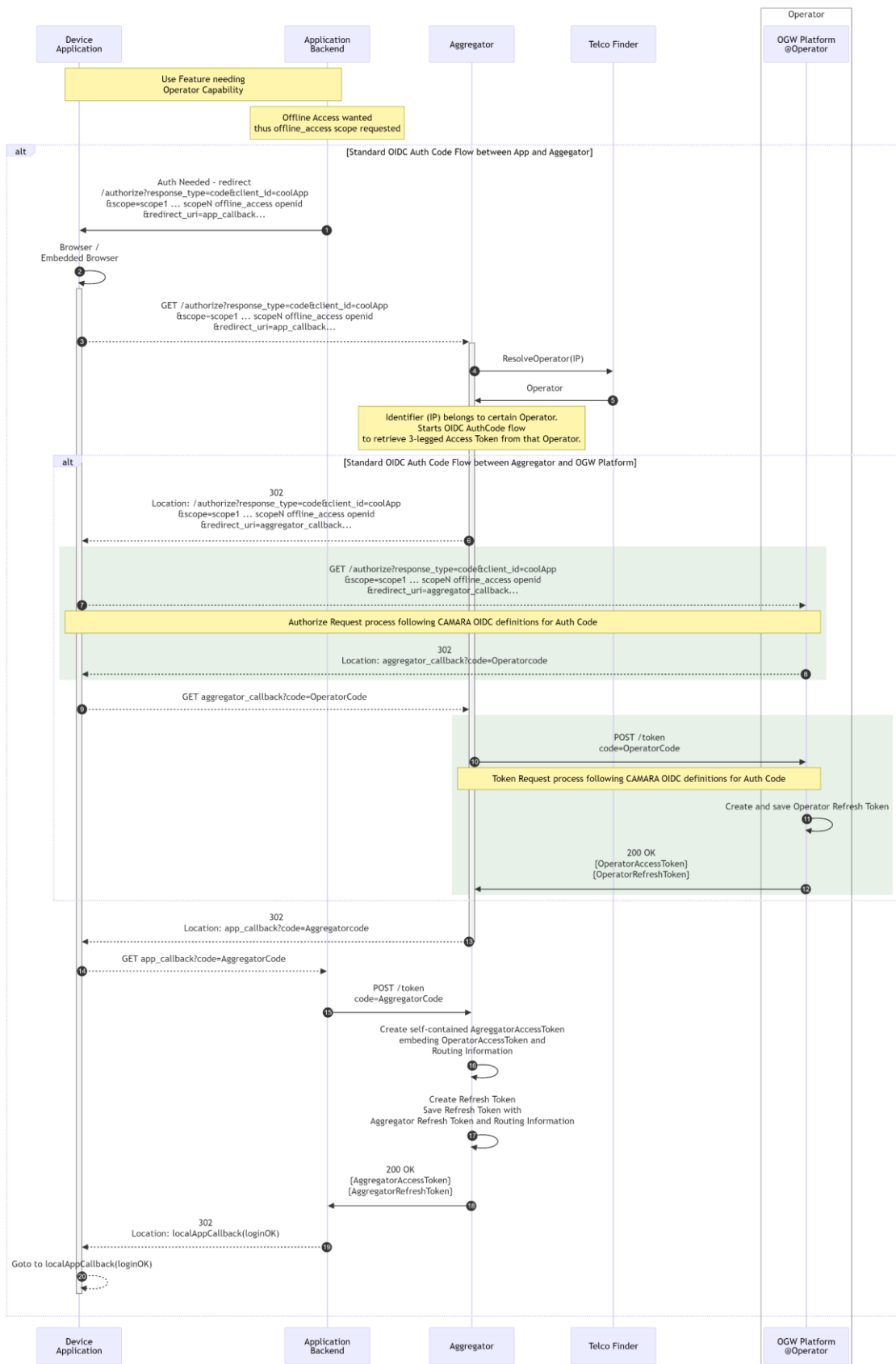
Figure 12: Request a Refresh Token in frontend-based flow
