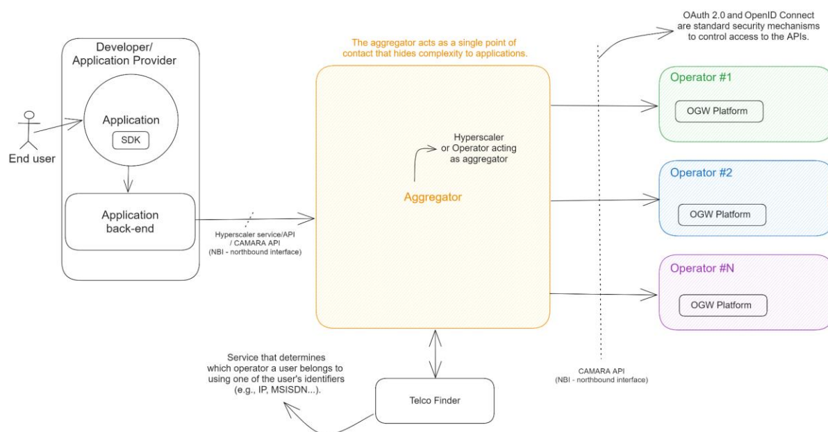
Figure 6: Aggregation model
