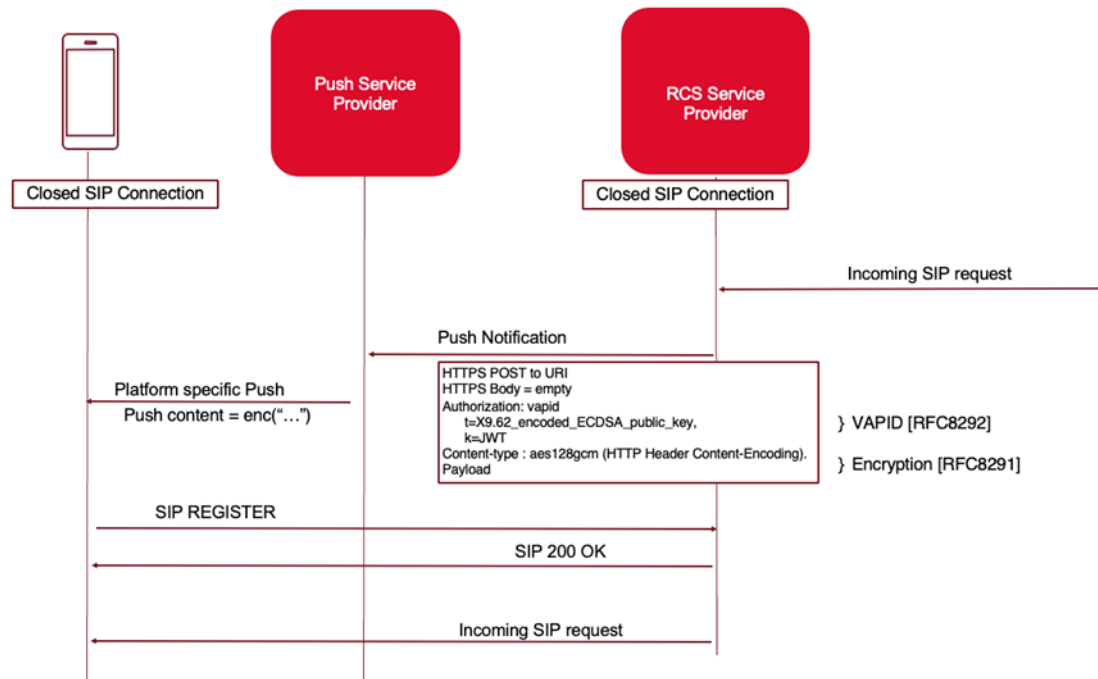
Figure 9: Push Notifications with content in HTTP body
