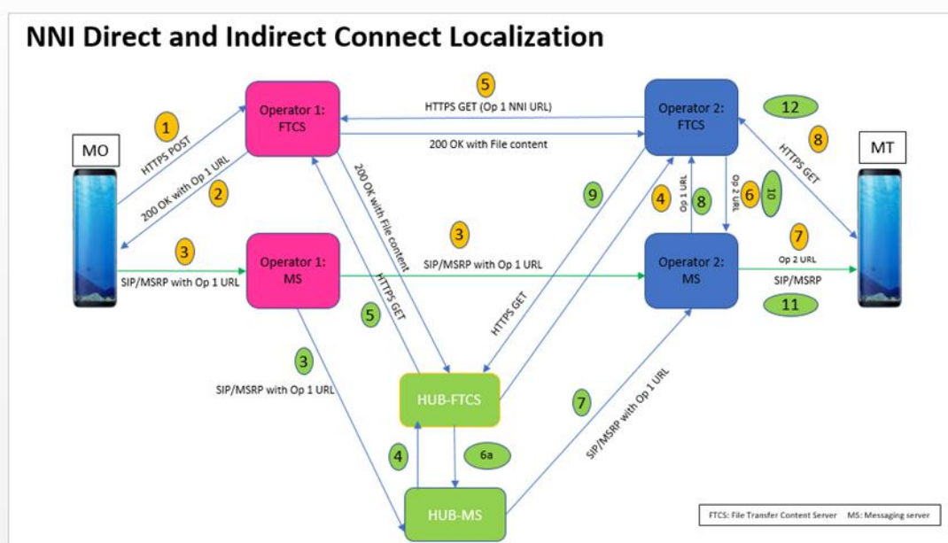
Figure 27: NNI Localisation with direct and indirect connections
