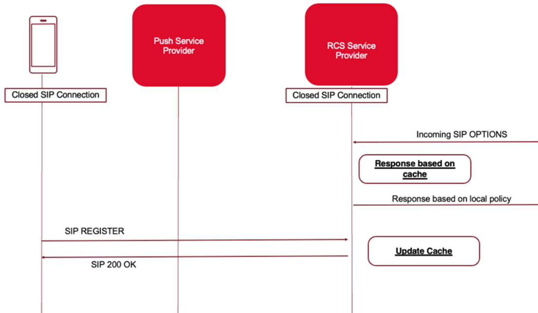
Figure 10: Capability discovery and cache behaviour for Push Notification
