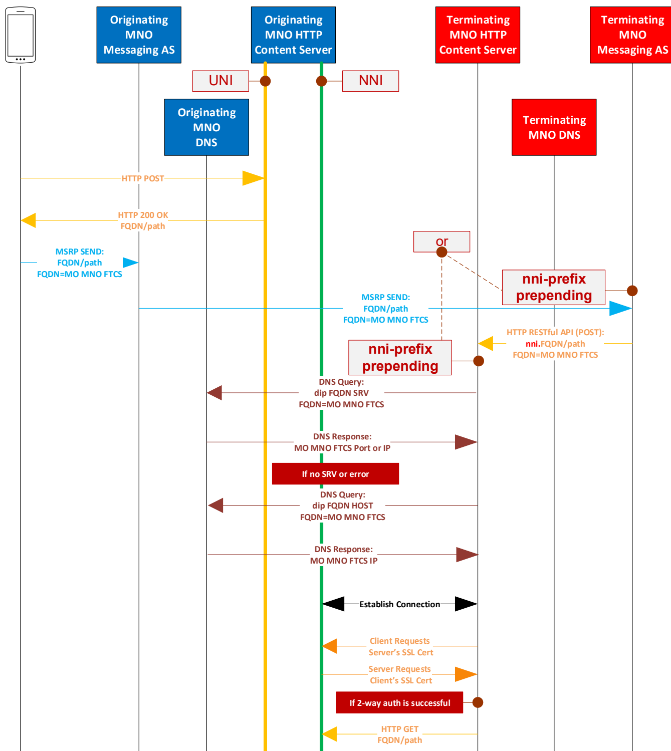
Figure 26: Mutual Authentication for HTTP File Transfer Localization Option 2 with Terminating MNO performing “nni-prefix prepending”
