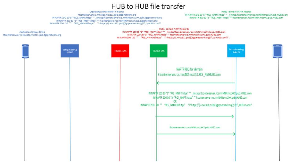
Figure 29: Mutual Authentication for HTTP File Transfer Localization Hub to Hub transfer (Part 2)
