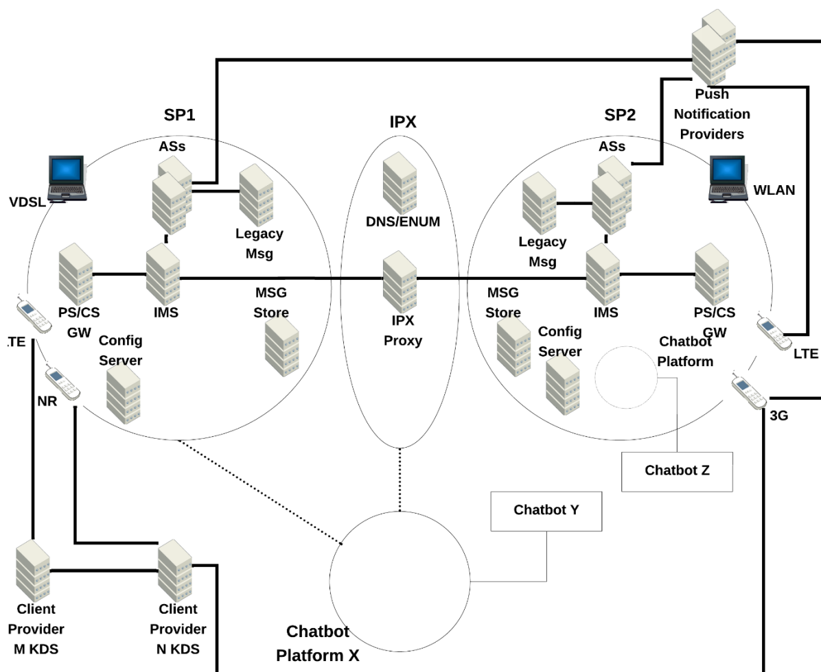
Figure 1: Simplified Example of RCS Architecture
