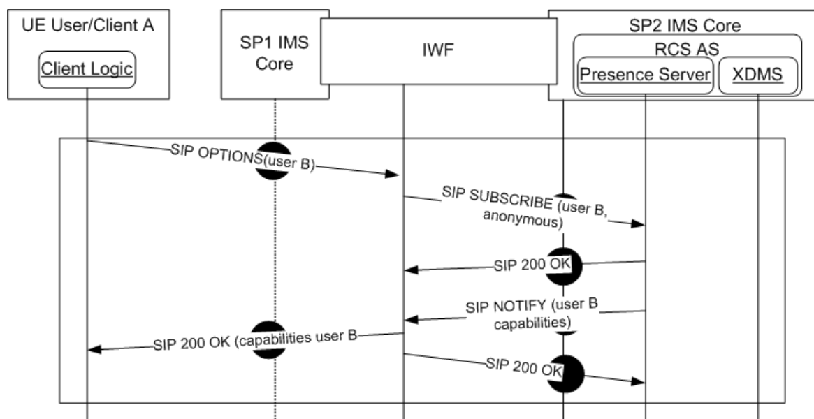
Figure 4: Capability Discovery interworking via network: Options request
