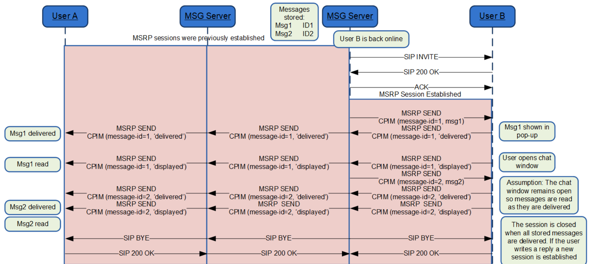
Figure 38: Store and forward: Message(s) deferred delivery with a sender still on an MSRP session*
