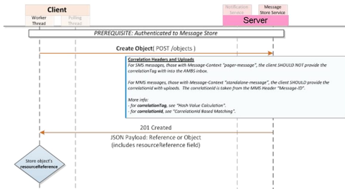
Figure 48: Message Store – Object Upload
