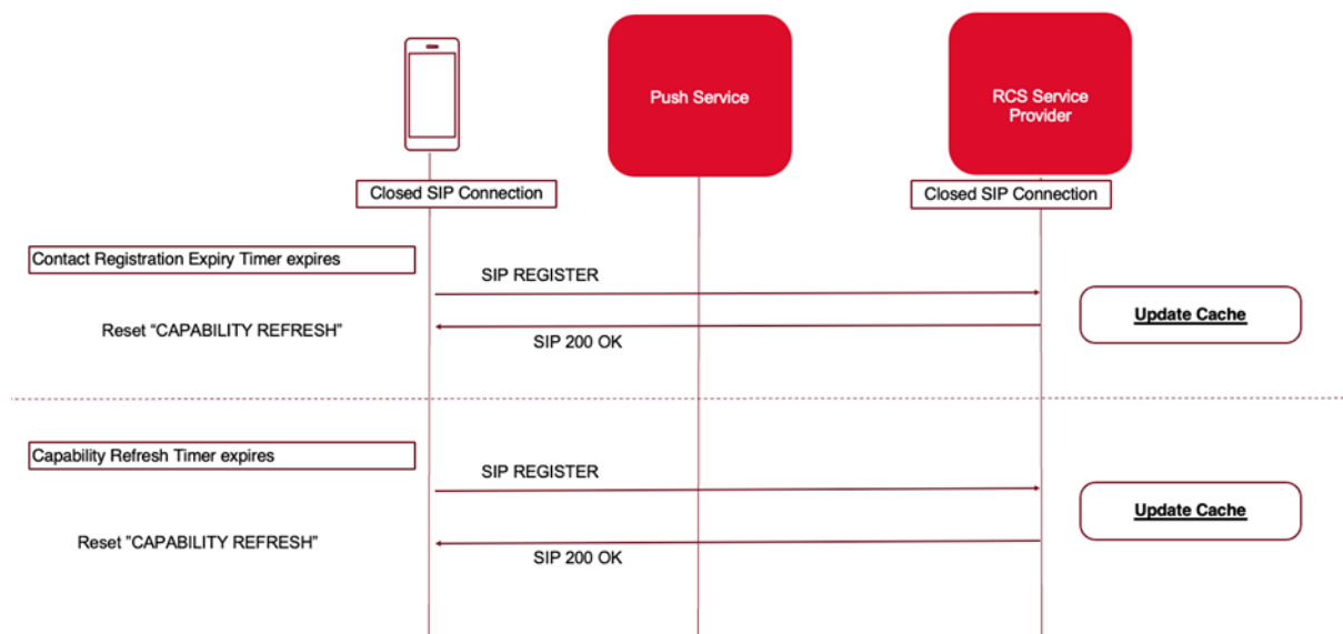
Figure 11: CAPABILITY REFRESH and cache
