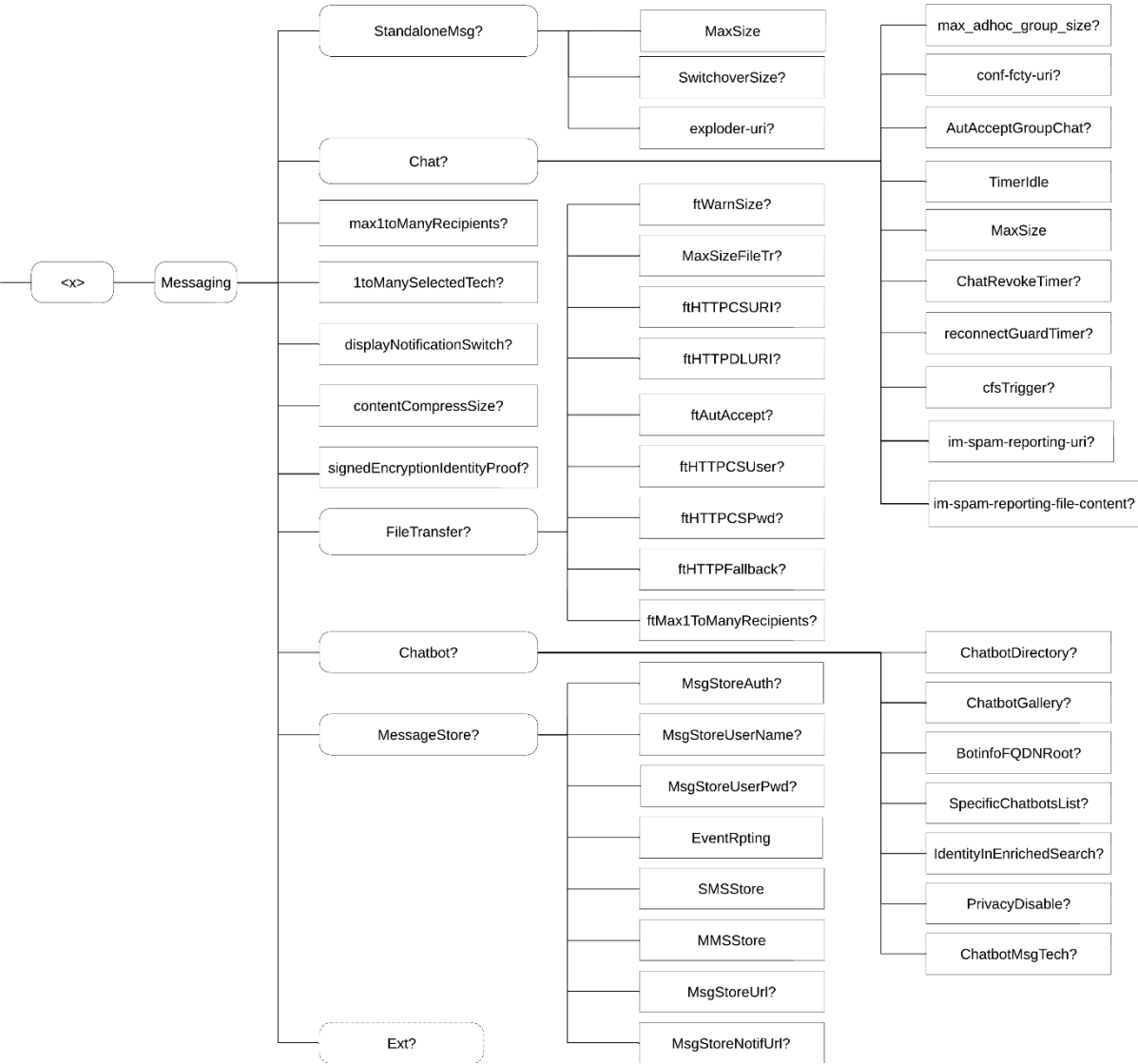
Figure 33: RCS additions to the IM MO sub tree
