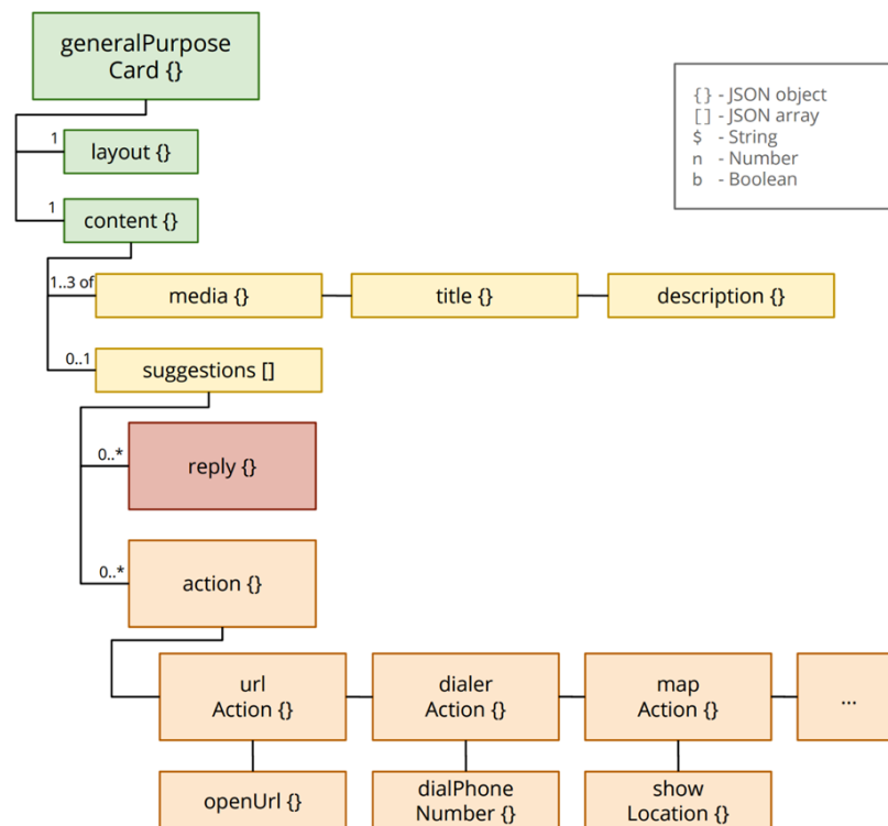
Figure 19: JSON Single Rich Card data structure overview
