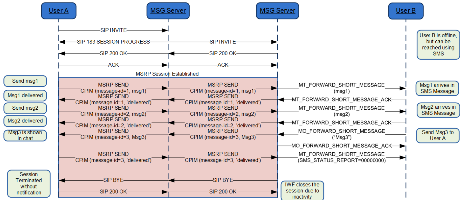
Figure 42: Interworking: Automatic acceptance on behalf of the SMS/MMS user*
