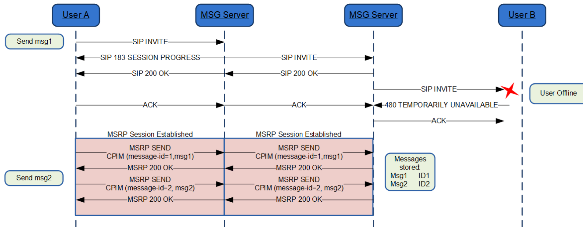
Figure 37: Store and forward: Receiver offline*
