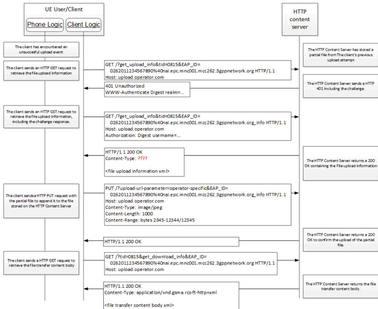
Figure 31: File Upload Resume
