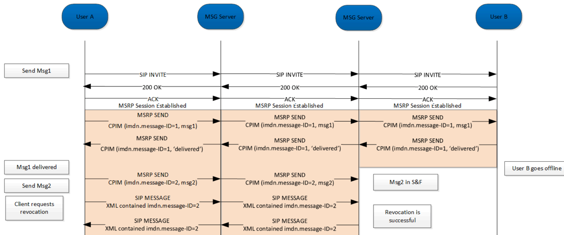
Figure 43: Message Revoke, Successful request*
