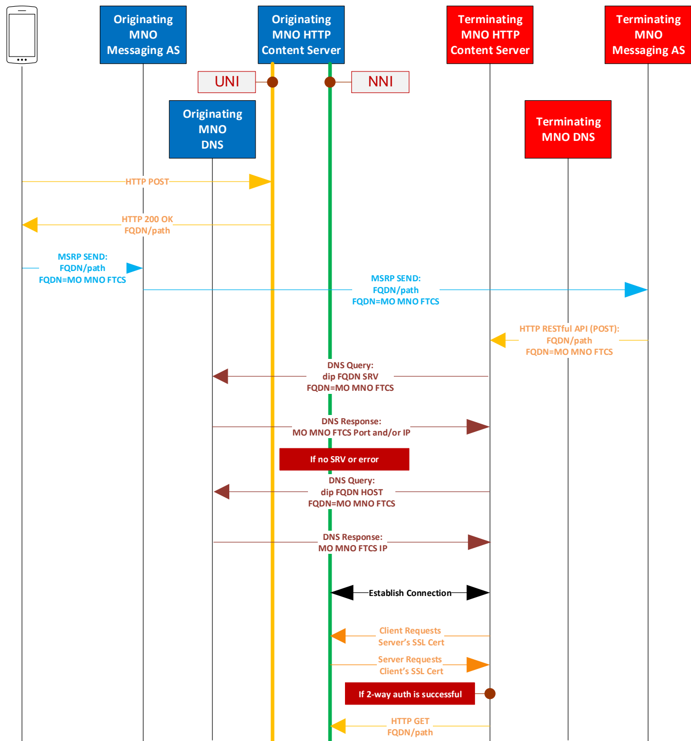
Figure 24: Mutual Authentication for HTTP File Transfer Localization Option 1 (SRV based)
