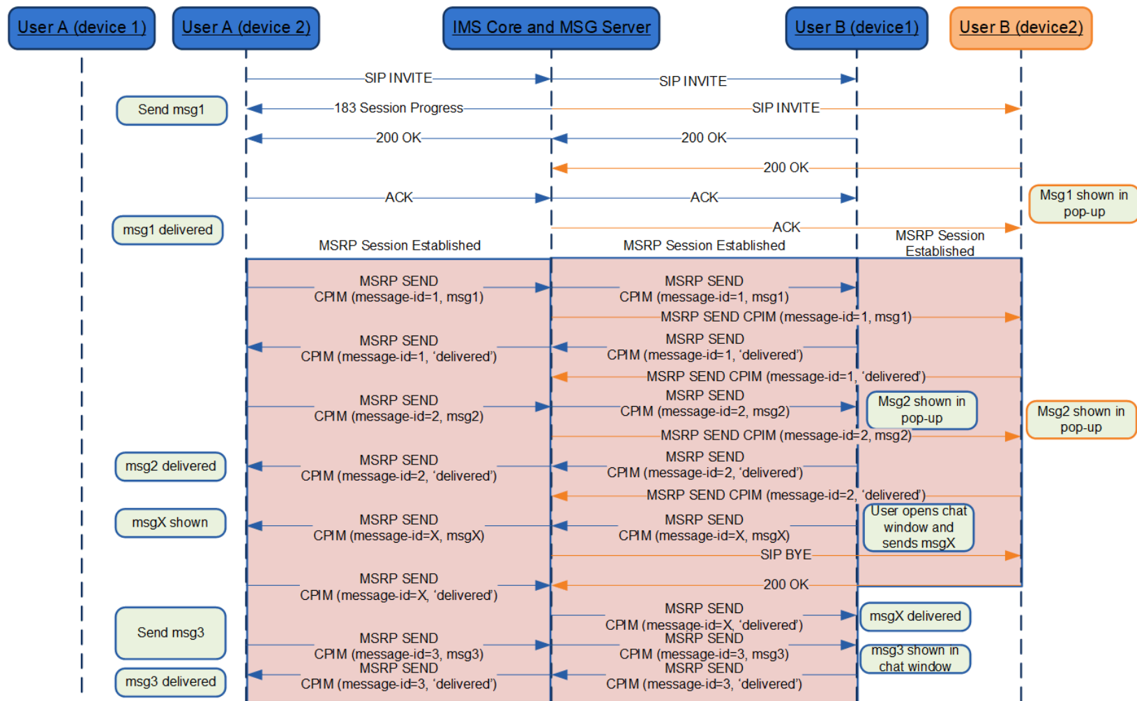
Figure 46: Rejoin in active Chat which is torn down due to inactivity*
