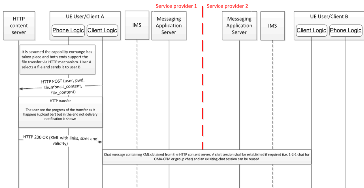
Figure 12: File Transfer: Sender procedures
