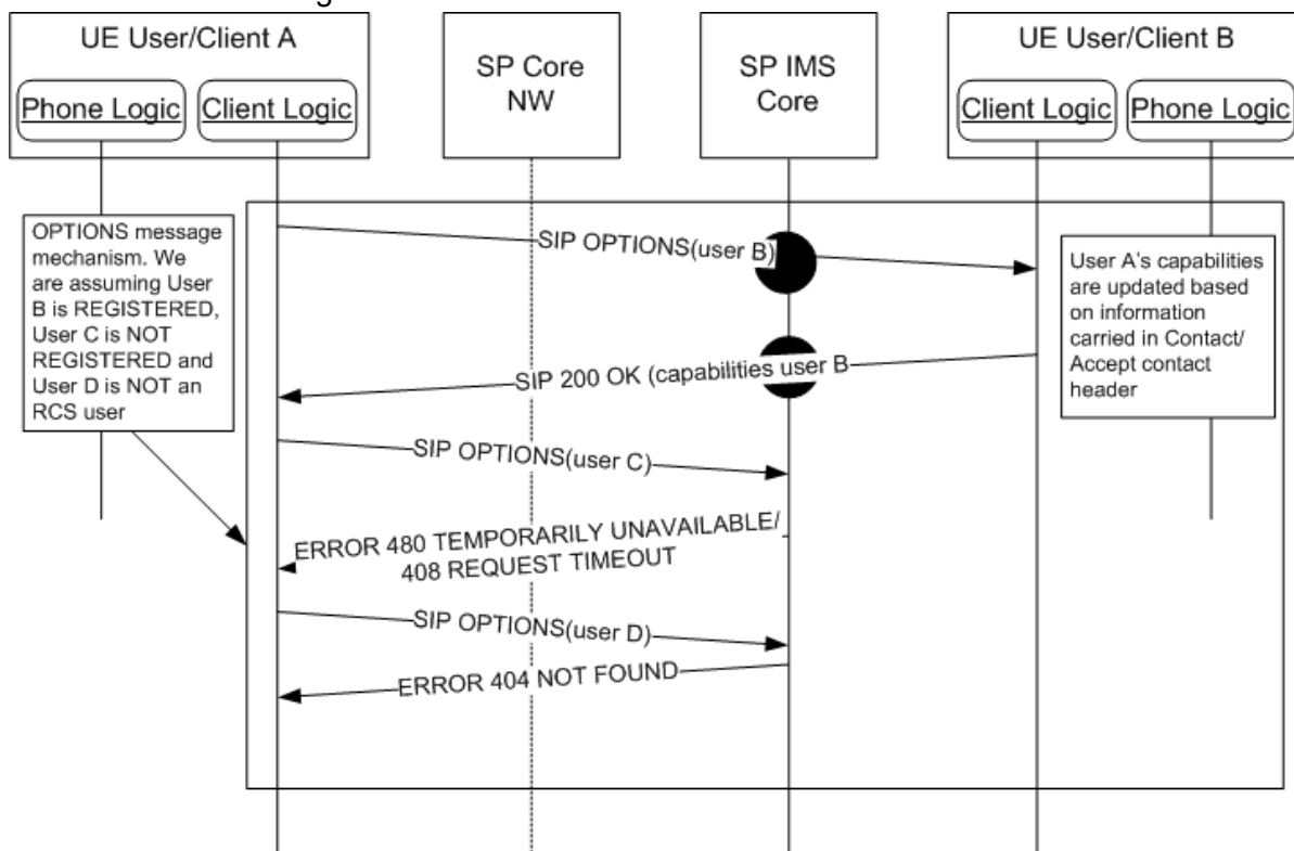
Figure 2: Capability Discovery via SIP OPTIONS message
