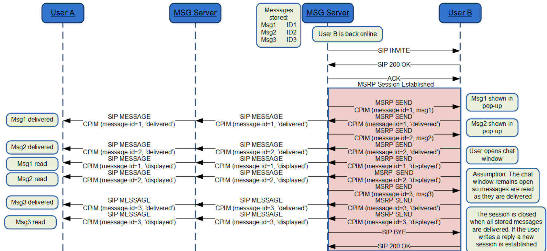
Figure 39: Store and forward: Message deferred delivery with sender online *
