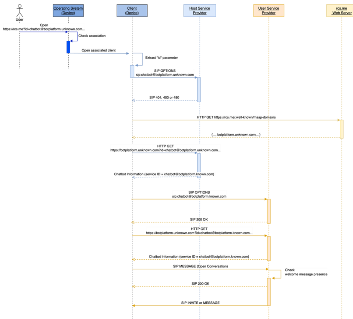
Figure 17: rcs.me fallback via alternative Chatbot service identifier
