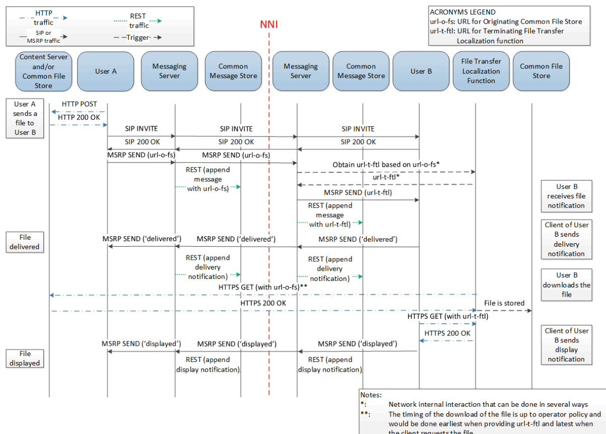
Figure 23: File Transfer Localisation Function: global flow
