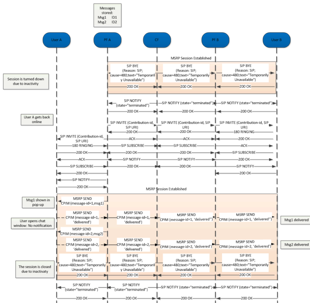
Figure 45: Deliver Group Chat Messages while Chat is idle*
