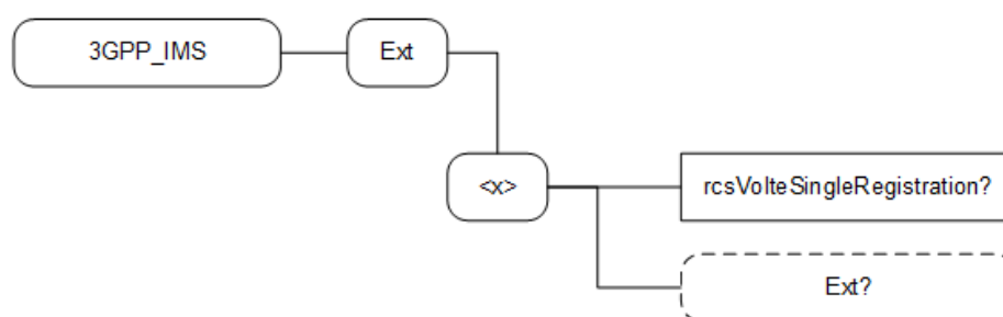
Figure 36: Additions to the IMS MO sub tree
