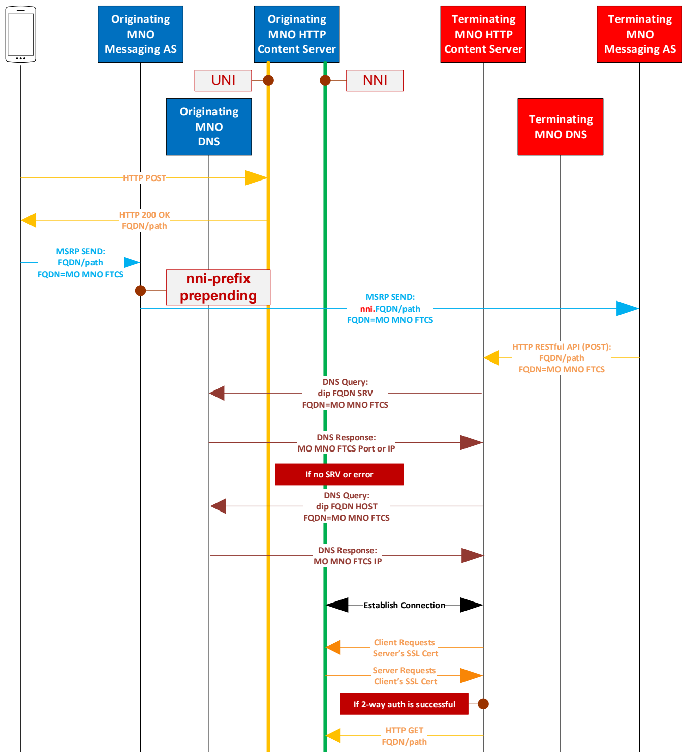
Figure 25: Mutual Authentication for HTTP File Transfer Localization Option 2 with Originating MNO performing “nni-prefix prepending”
