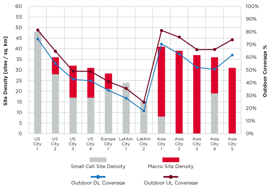
Figure 1: 5G mmWave coverage for different site densities worldwide
