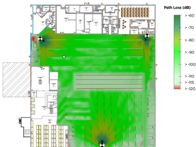
Figure 6: 5G mmWave coverage in an industrial environment
