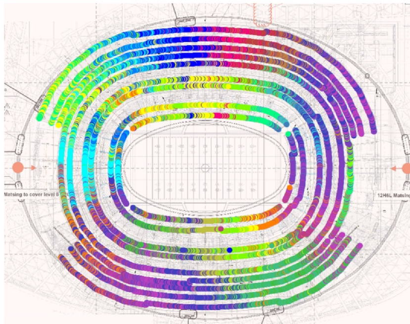
Figure 4: Best PCI plot of a mmWave deployment in a stadium in North America
