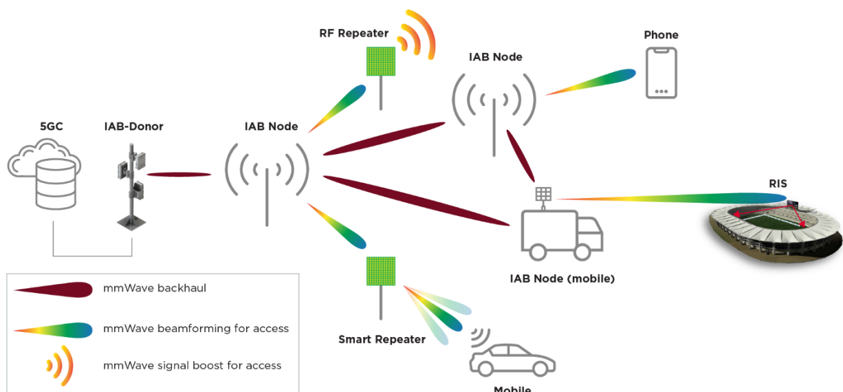
Figure 8: An overview of different network nodes - IAB and repeater topology
