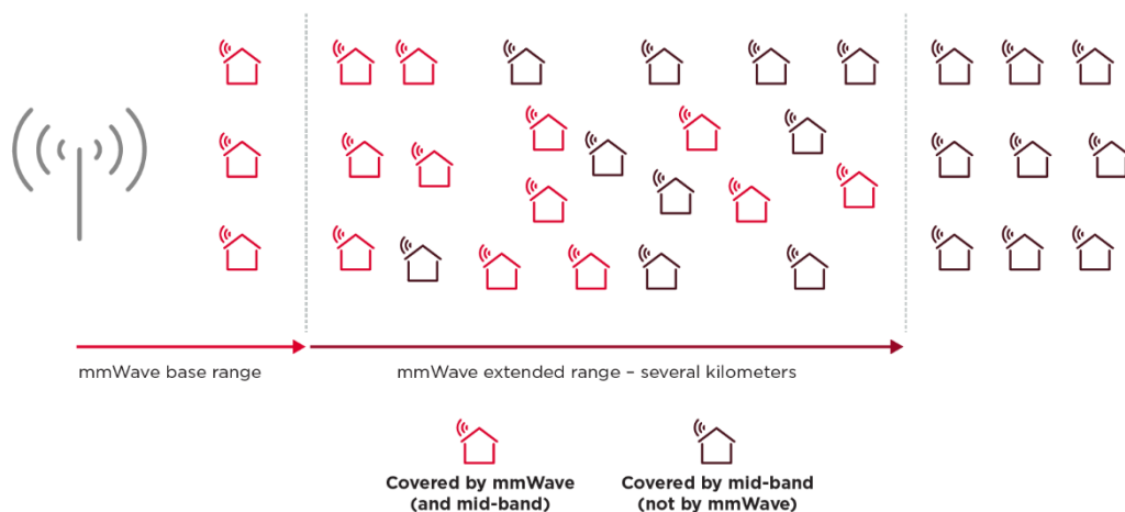
Figure 7: mmWave extended range can be used to provide FWA across several km
