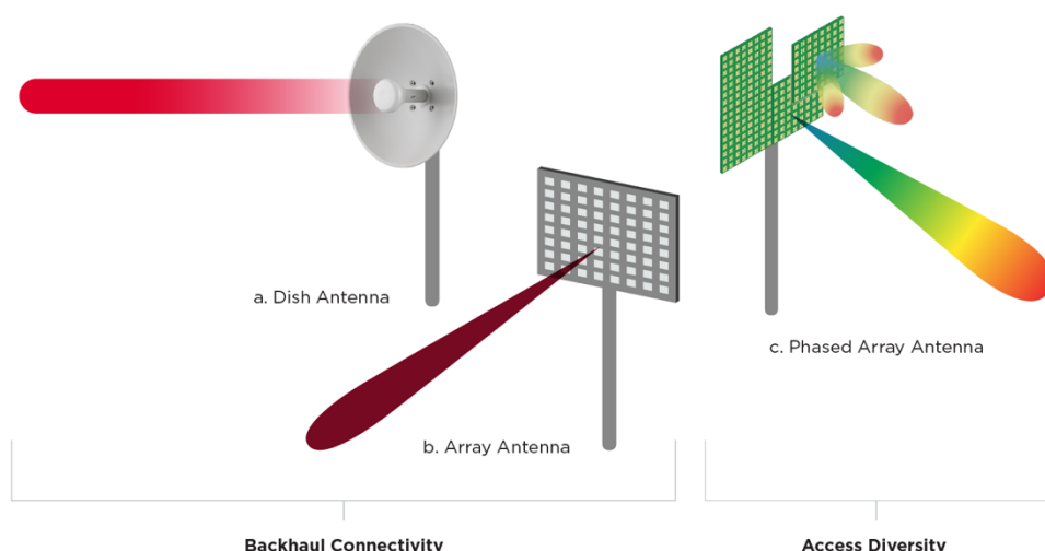
Figure 10: Different antenna types for backhaul and access
