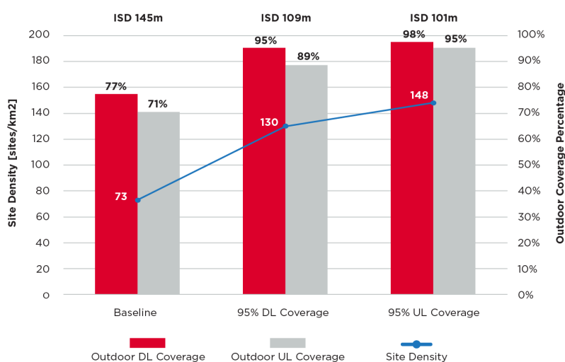
Figure 2: 5G mmWave coverage improvement via densification
