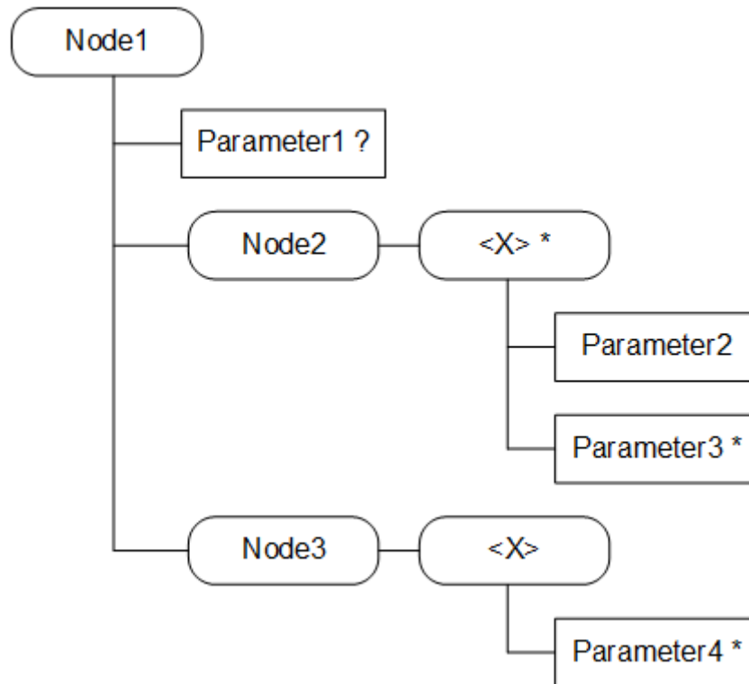
Figure 20: Example MO Tree
