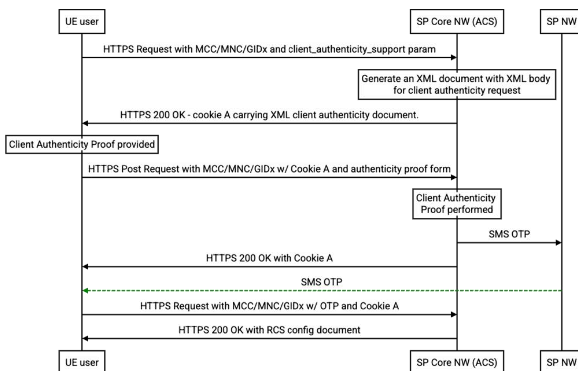
Figure 16: Example Client Authenticity Verification Flow
