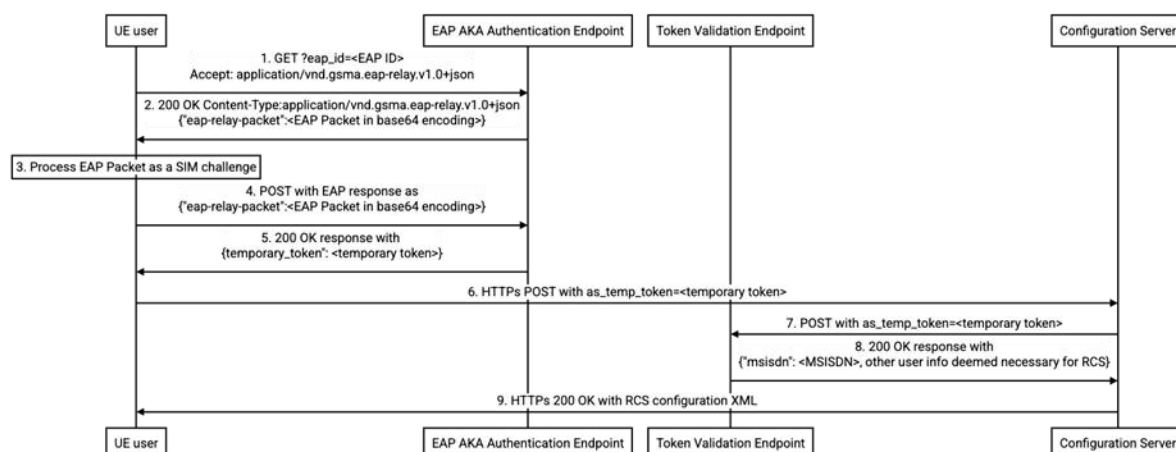
Figure 21: configuration using Temporary Token end-to-end flow
