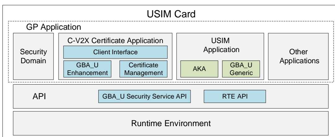
Figure 7: USIM Card Architecture
