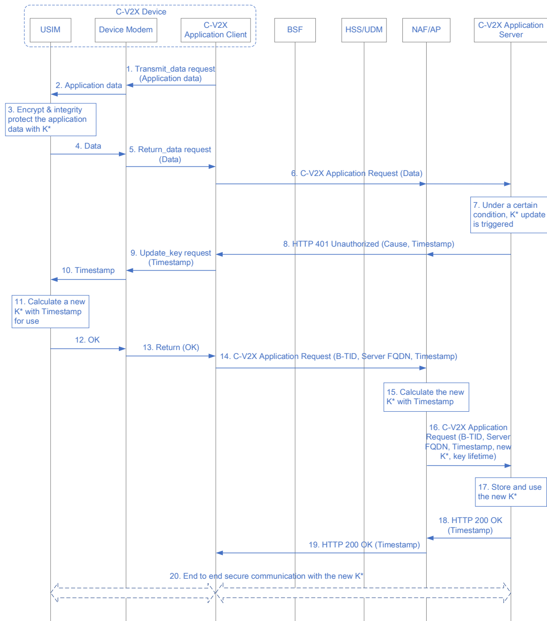
Figure 8: K* renegotiation procedure for Solution 2
