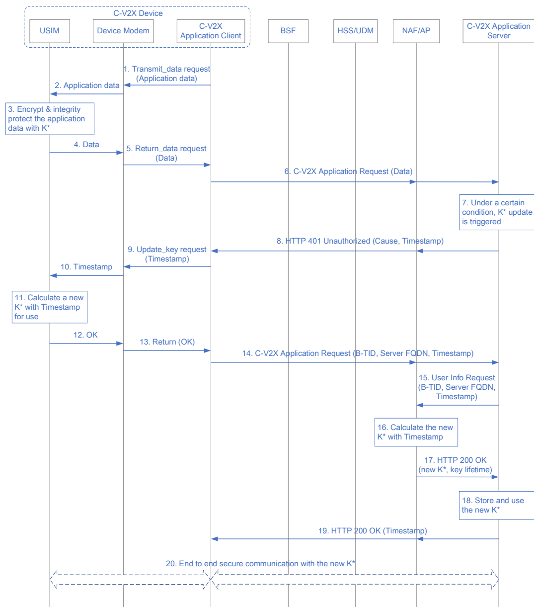
Figure 7: K* renegotiation procedure for Solution 1
