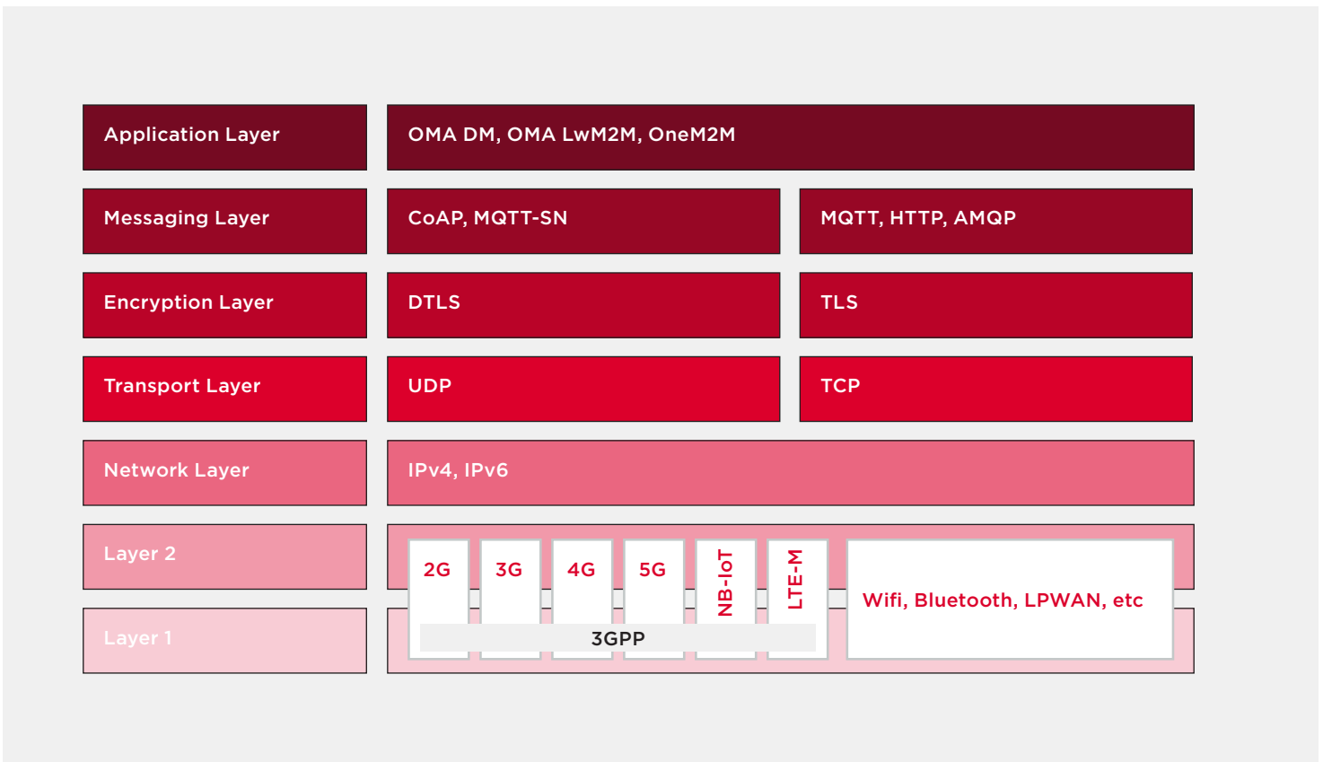
Figure 4, Commonly used Protocols
