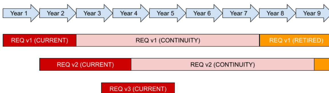
Figure 2 – Requirements Lifecycle
